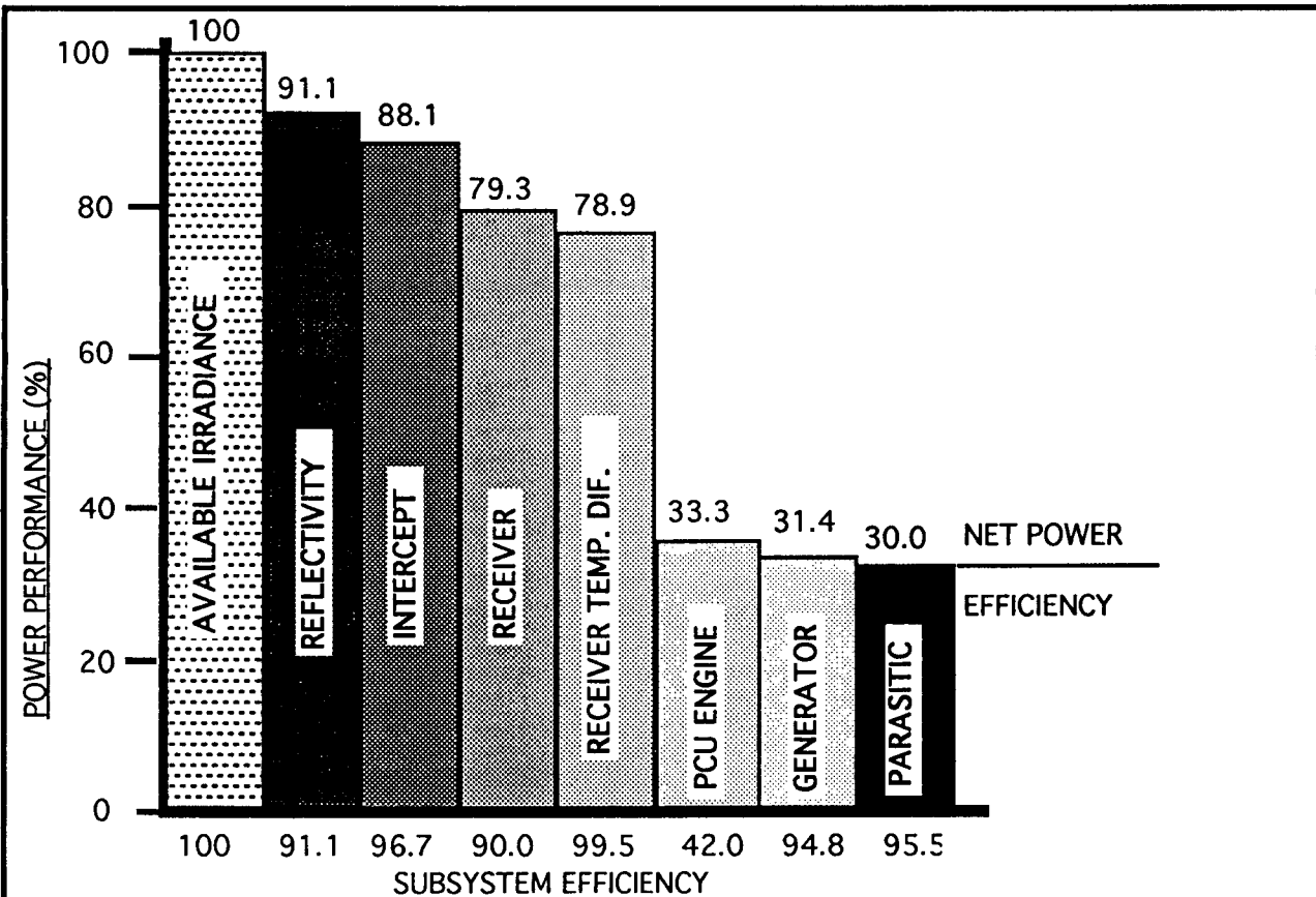
Figure III-6. System and Subsystem Peak Power Efficiency.
