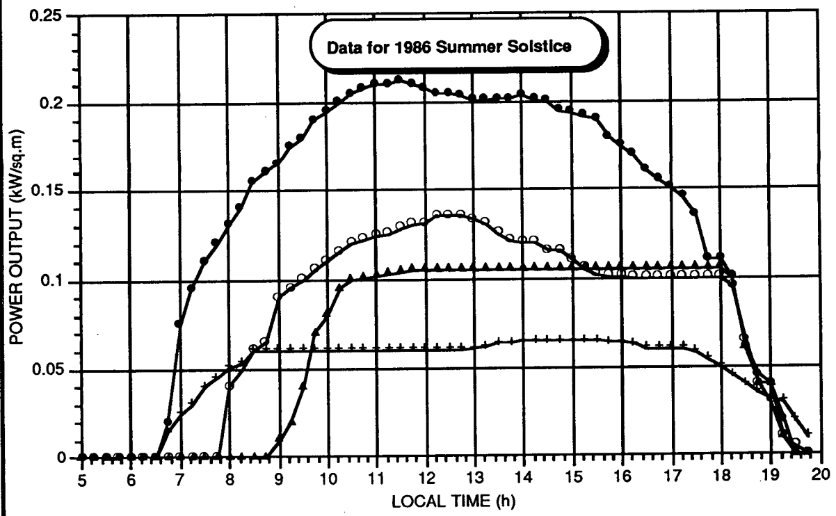
Figure V-1. Power Comparison of the Stirling Dish, Solar One, Intersol PV and SEGS 3.
