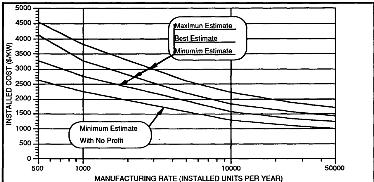
Figure VIII-6. Installed Cost of the Stirling Dish System.
