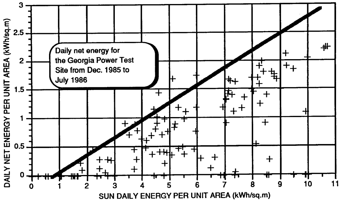
Figure IV-3. Energy Performance Test Data From the Georgia Test Site.
