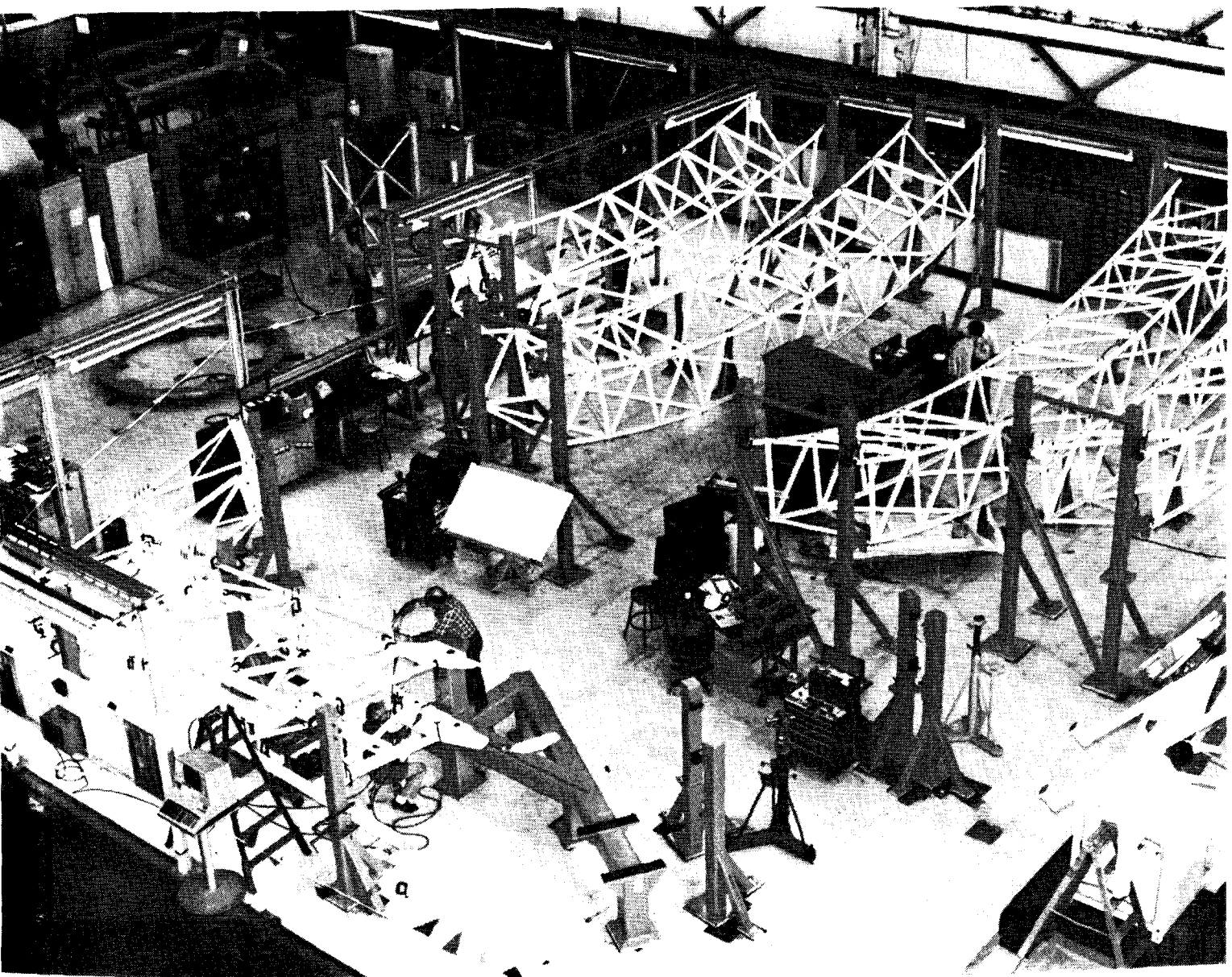
Figure II-6. Assembly of the Reflector and PCU Support Structure.
