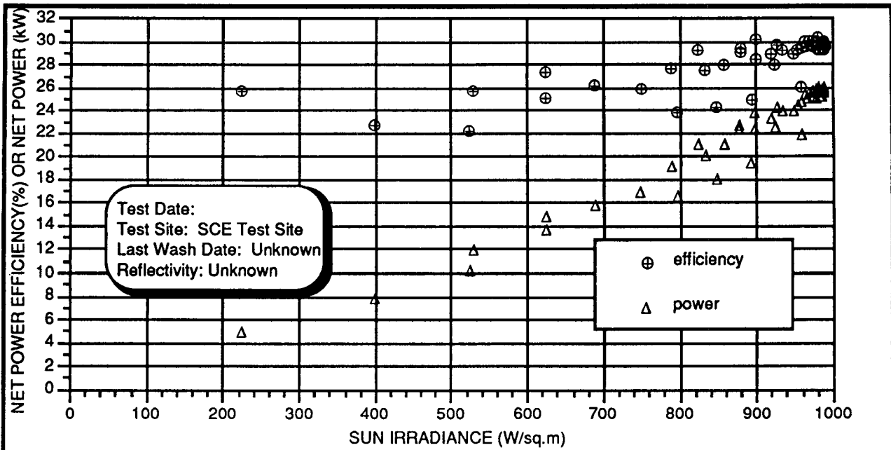
Figure III-5. Peak Power and Peak Power Efficiency at the SCE Test Site.
