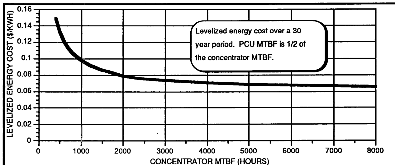
Figure VIII-7. Estimate of Levelized Energy Cost.
