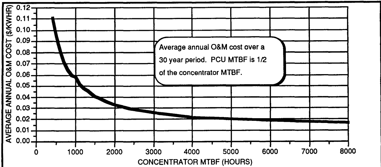
Figure VIII-8. Estimate of System O&M Cost.
