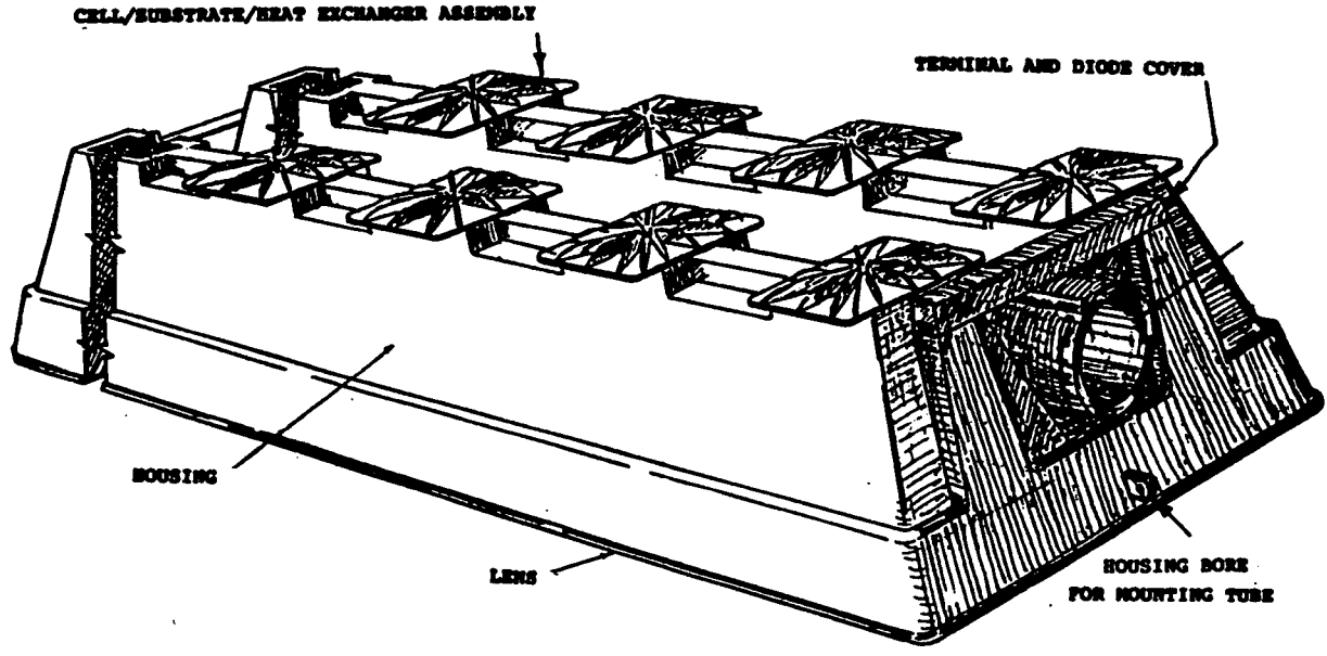
Figure V-6. Intersol PV Module Design.
