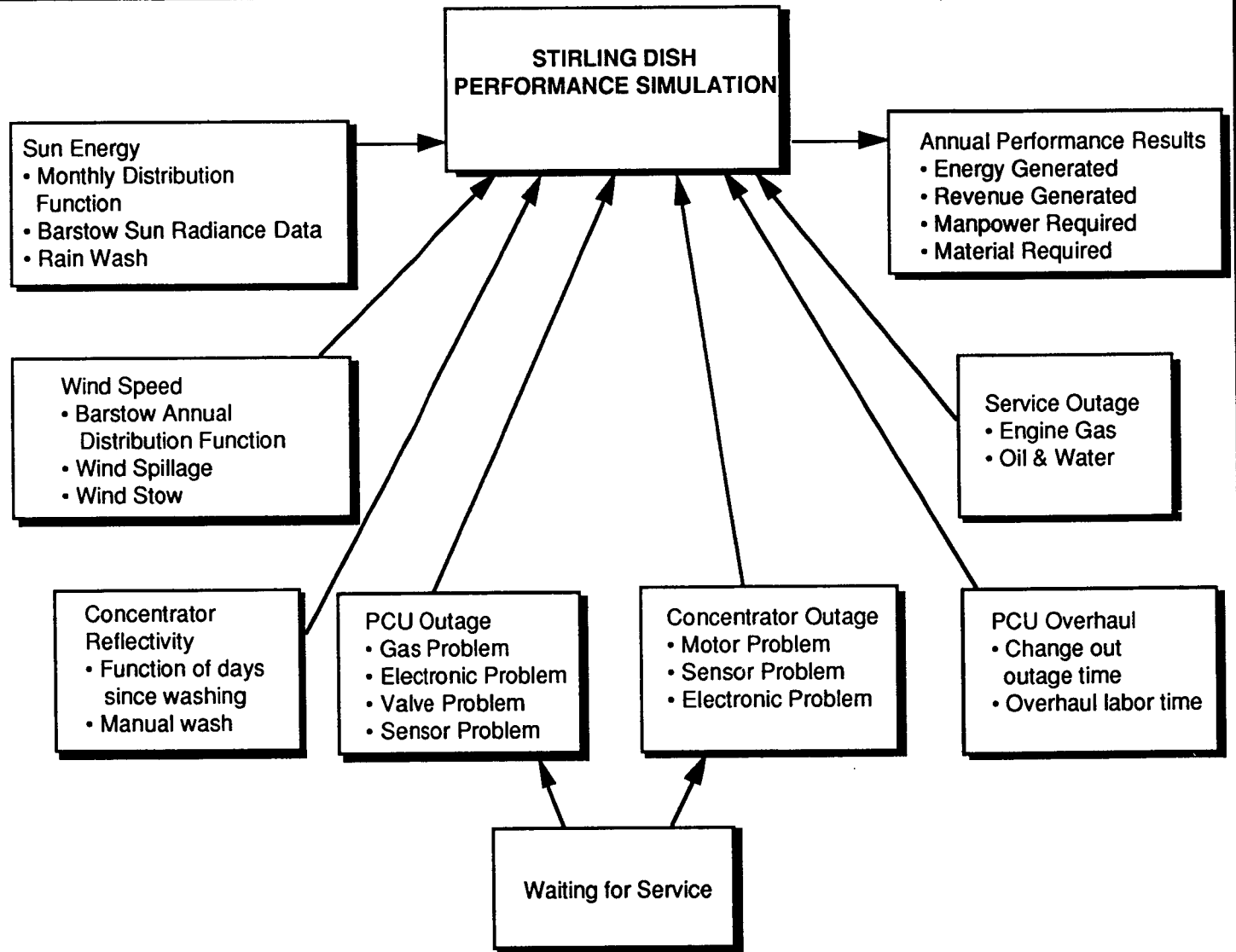
Figure VIII-1. Stirling Dish Annual Performance Simulation.
