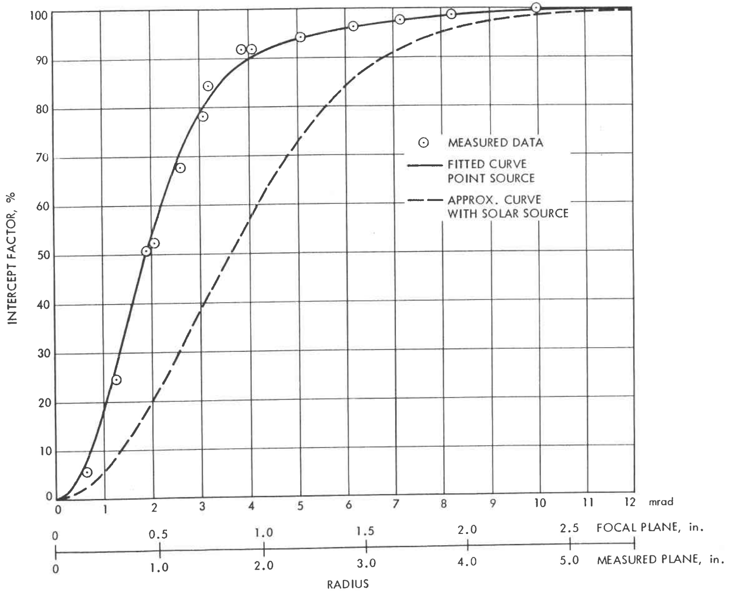
Figure 3. Intercept Factor Curve Using Measured Data
