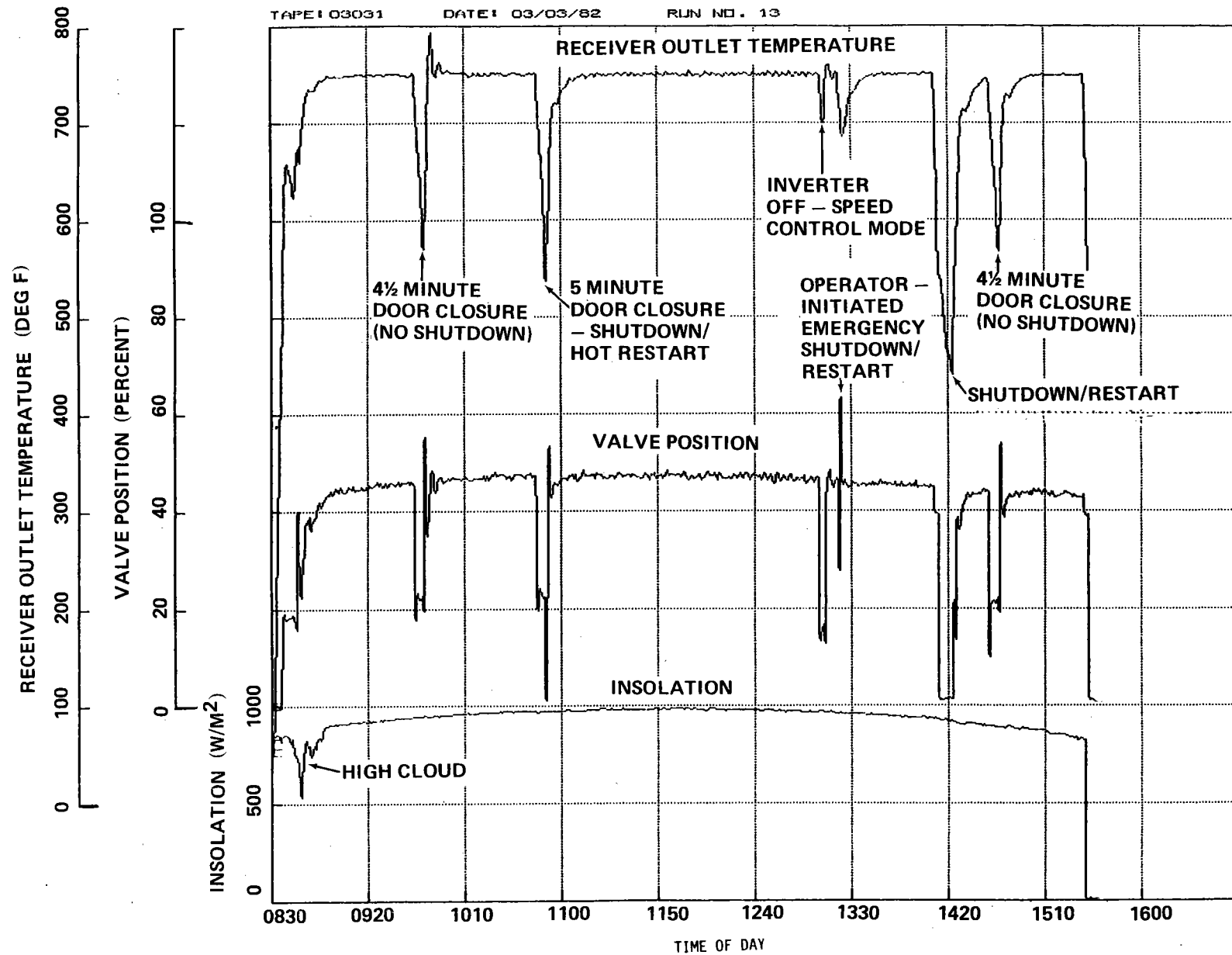
Figure 4-7. Receiver Fluid Outlet Temperature vs. Valve Position (Run 13, Test No. 8)
