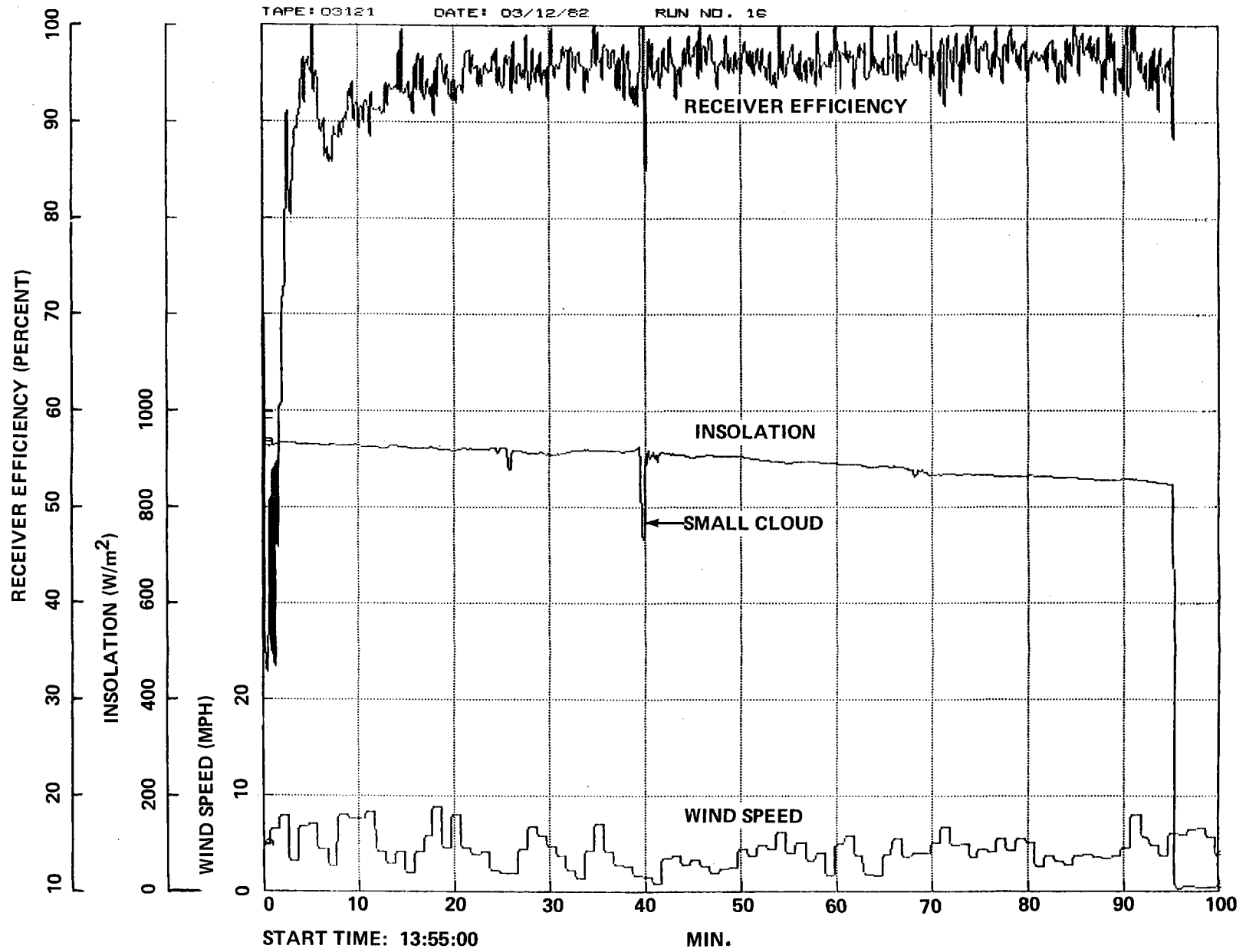
Figure 4-6. Typical Receiver Efficiency Plot (Run 16, Test No. 11)
