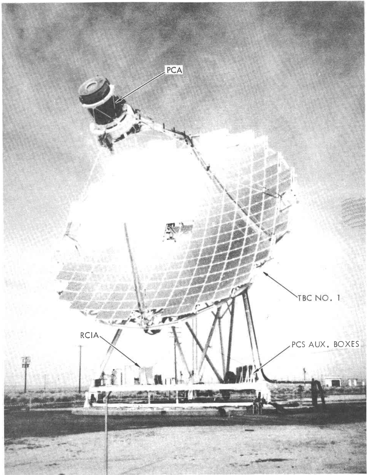
Figure 4-1. Power-Conversion Assembly and Electrical Boxes on Test Bed Concentrator No. 1
