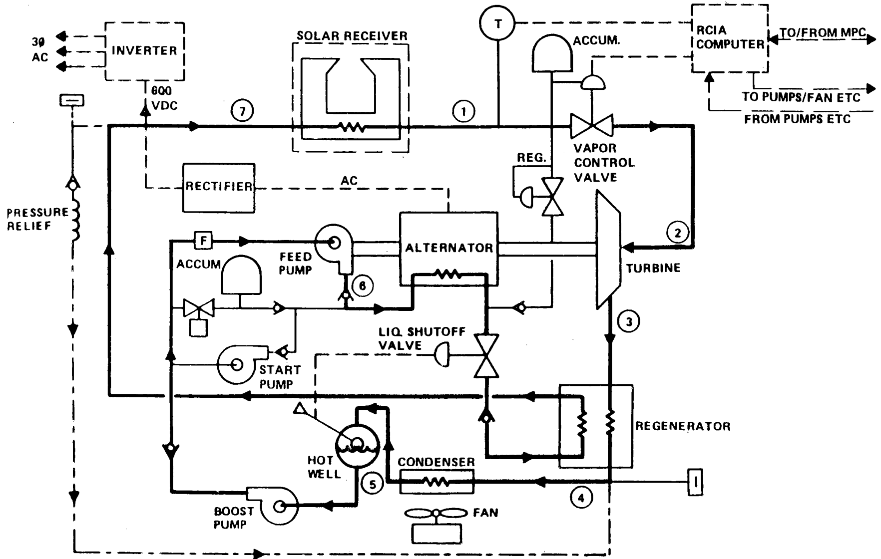
Figure 3-4. Schematic Diagram of ORC Power-Conversion Assembly. See Figure 3-5 for Temperature, Pressure, and Enthalpy of Working Fluid at Positions Identified by Circled Numbers.
