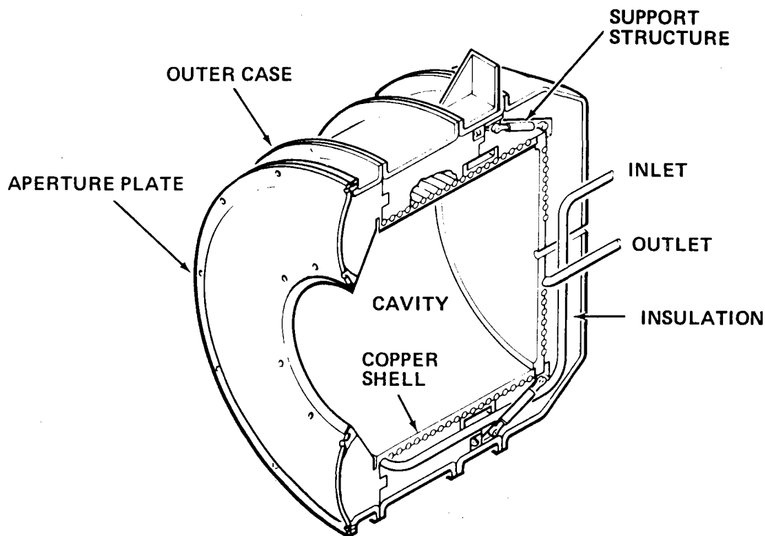
Figure 3-6. Cut-Away View of Receiver Assembly
