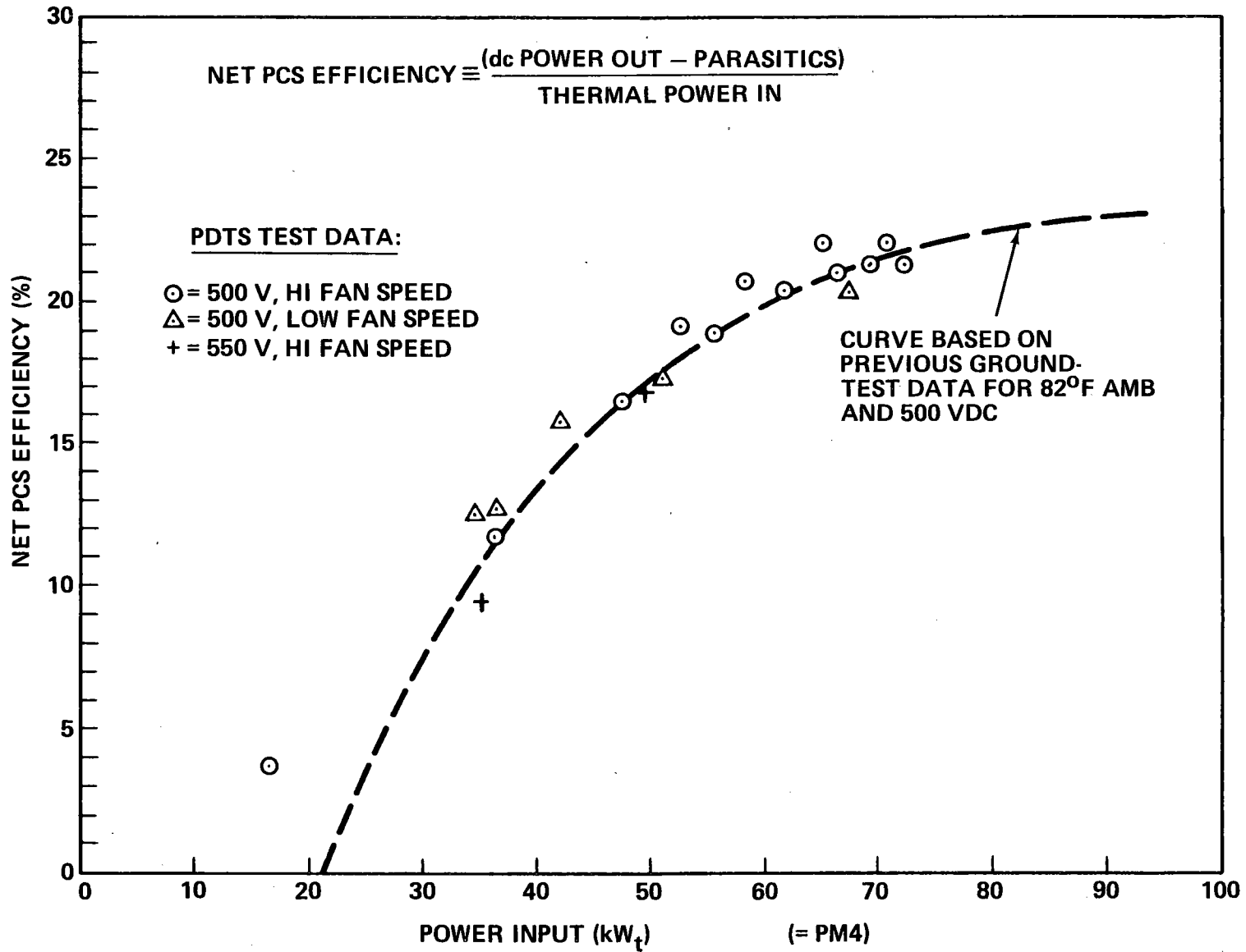
Figure 4-10. Measured ORC Engine Efficiency (Net after Parasitic Power Subtracted)
