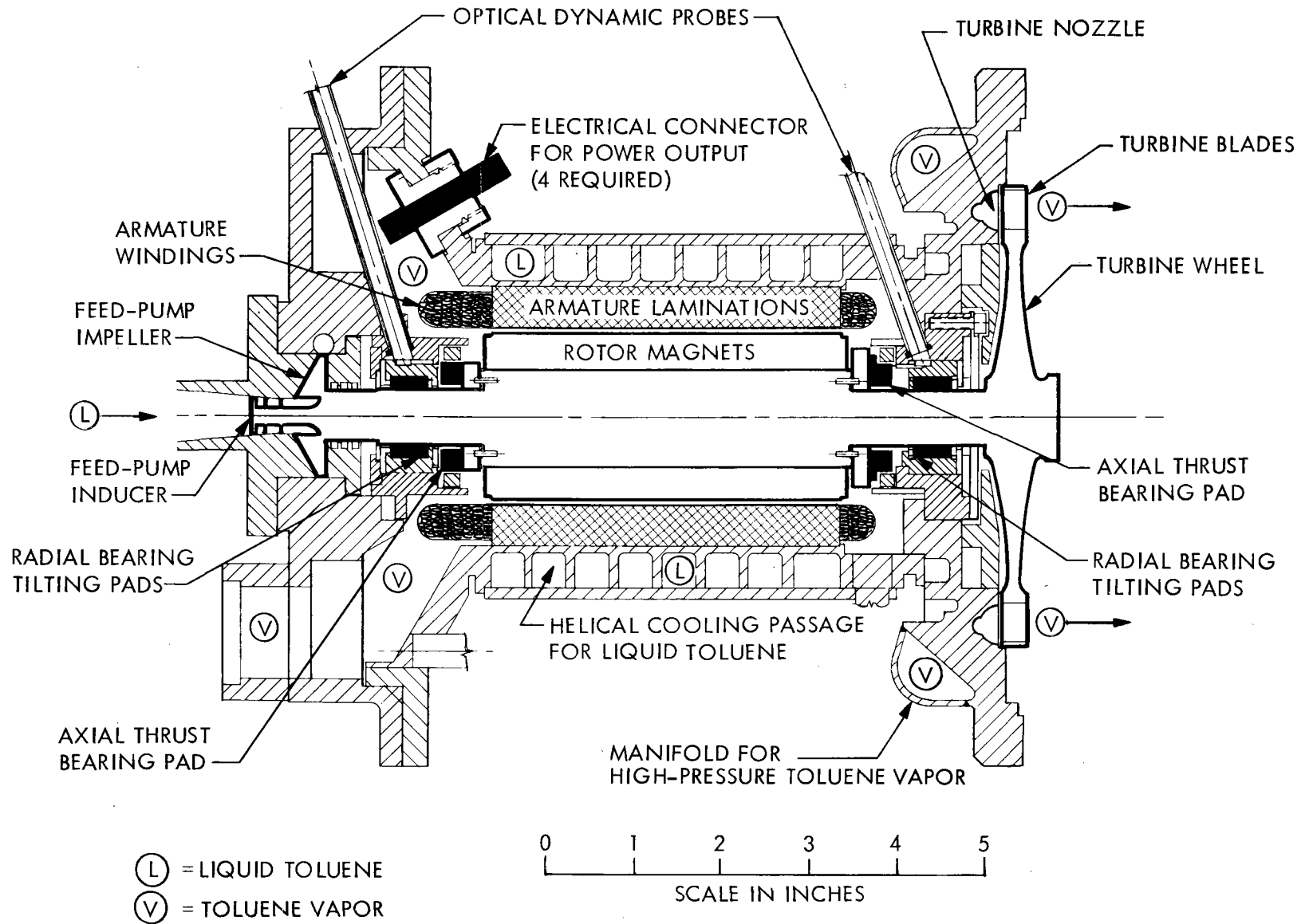
Figure 3-10. Cross-Section of TAP Assembly Showing, to Scale, Relative Sizes and Locations of Various Components
