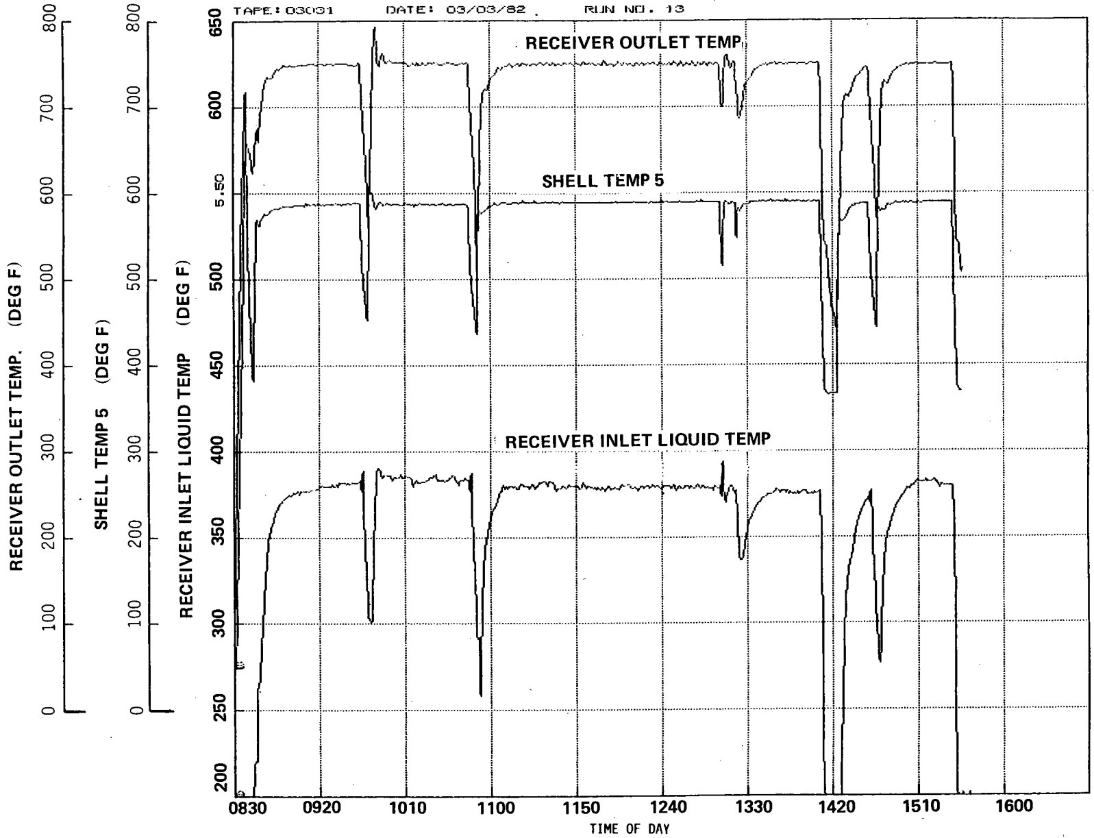
Figure 4-8. Receiver Temperatures for Run 13 (Test No. 8)
