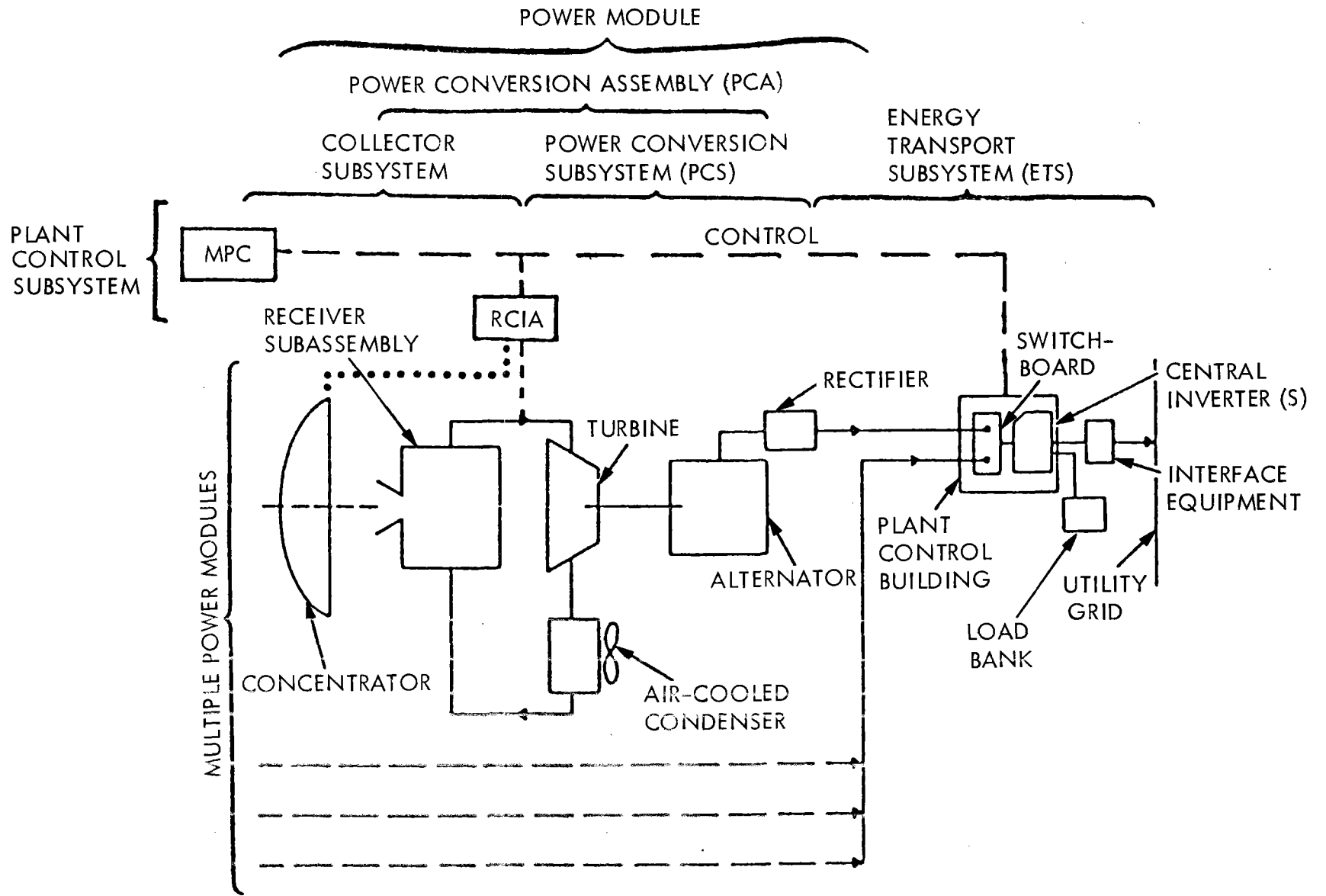
Figure 2-1. SCSE System Schematic (Power Plant)
