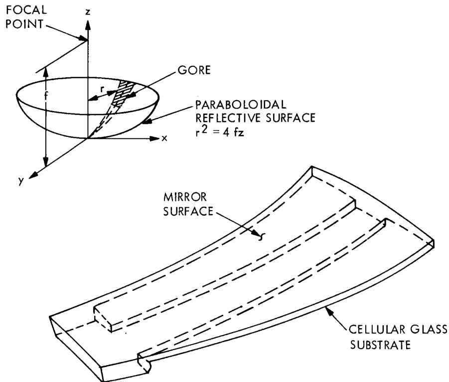
Figure 3-2. Mirrored Cellular Glass Gore
