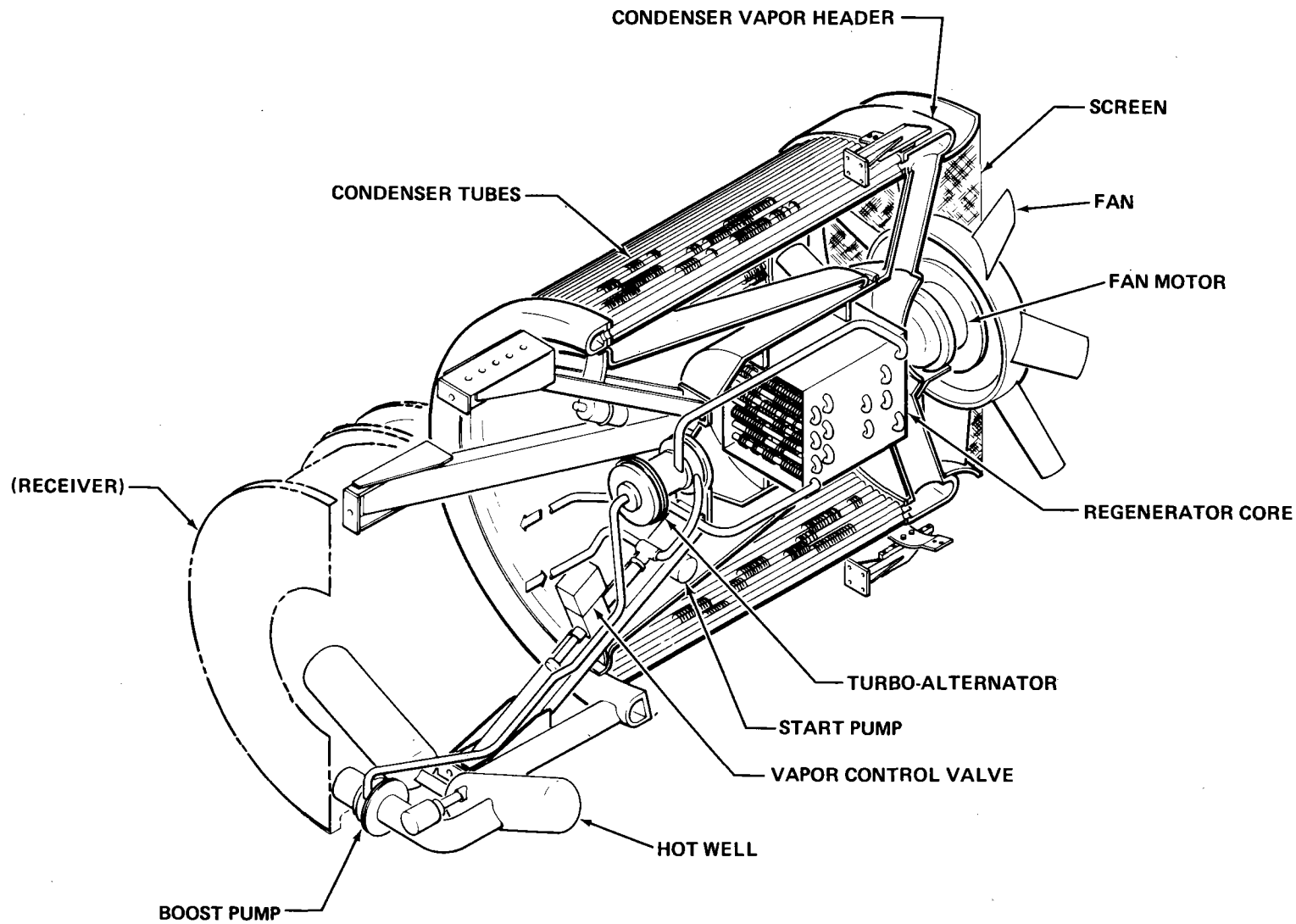
Figure 3-3. Power-Conversion Subsystem
