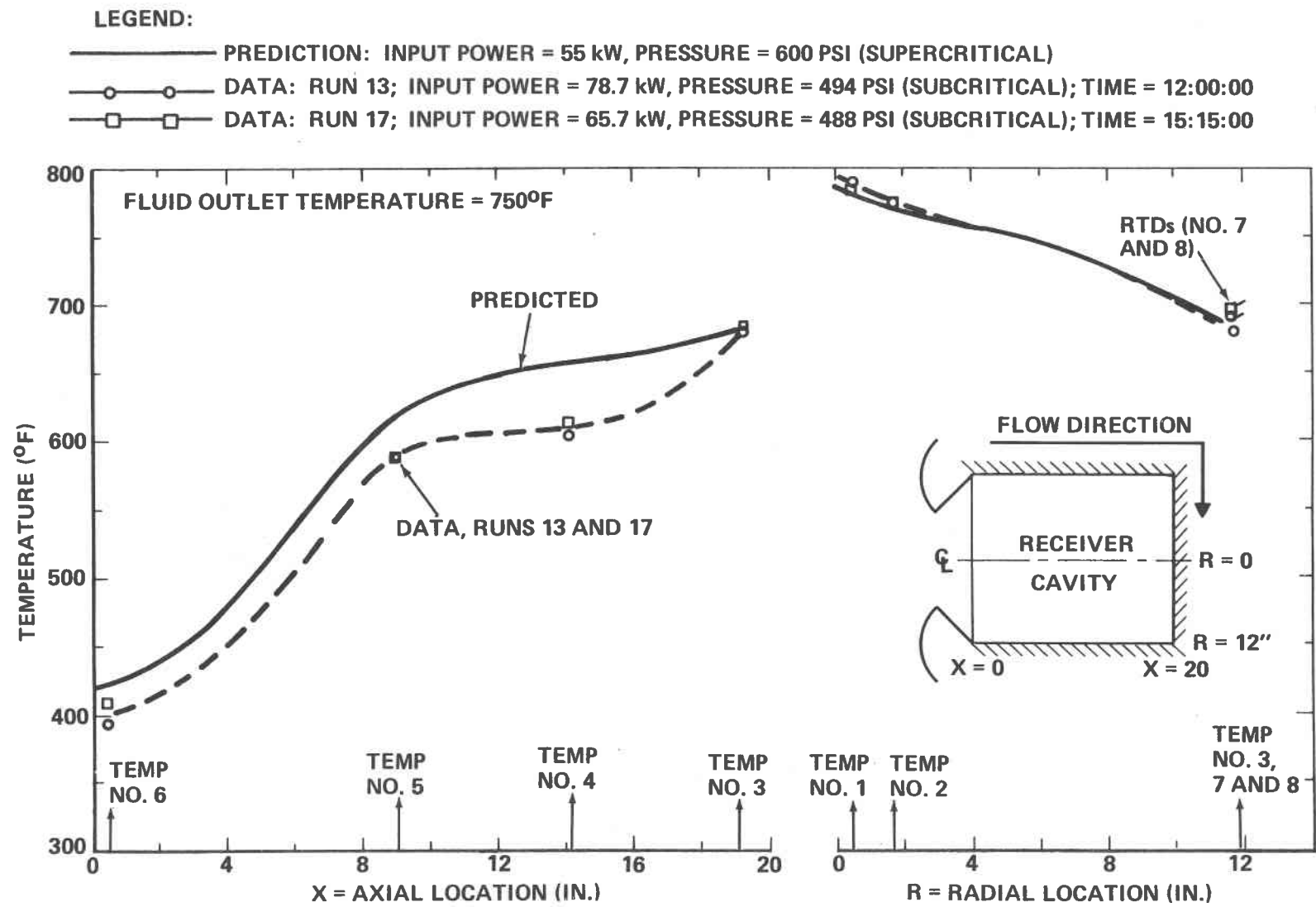
Figure 4-2. Comparison of Predicted and Measured Receiver Wall Temperatures (Runs 13 and 17)
