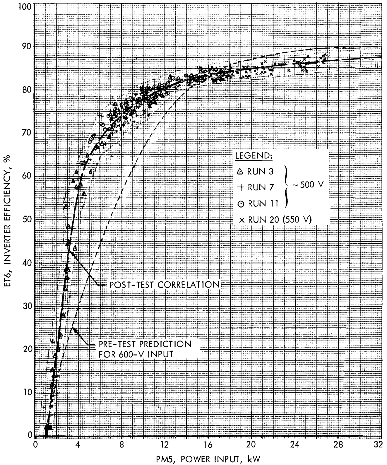
Figure 4-11. Inverter Efficiency Data and Pre-Test Predictions
