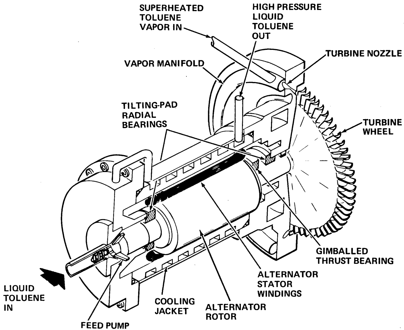
Figure 3-7. Turbine/Alternator/Pump (TAP) Assembly
