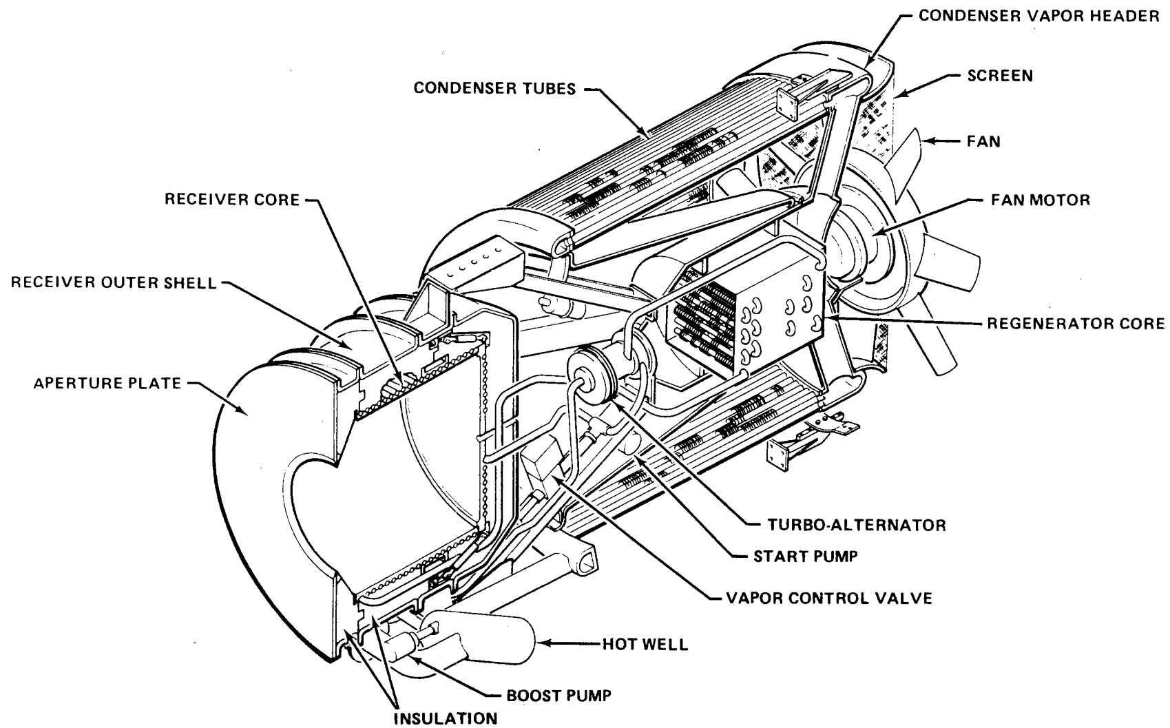
Figure 2-3. Power-Conversion Assembly (PCA)
