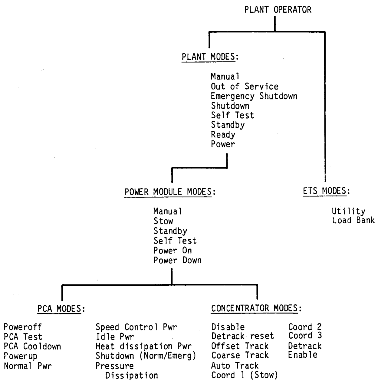
Figure 3-13. Typical Plant Moding Hierarchy
