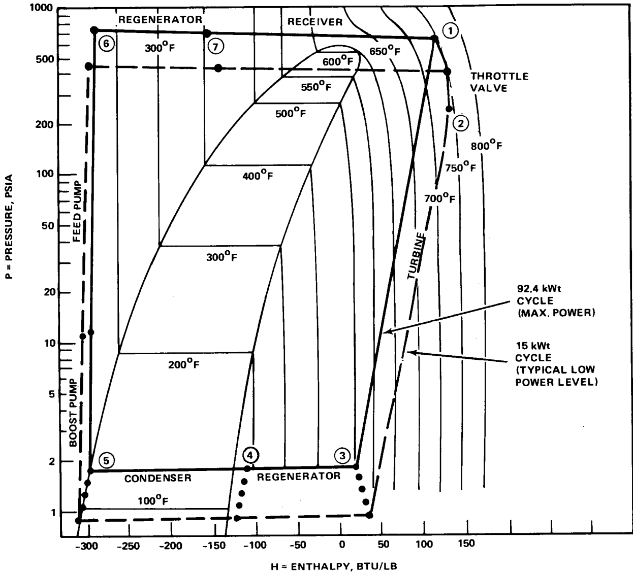
Figure 3-5. Diagram of Pressure/Enthalpy for the Organic Rankine Cycle. Numbers Designating State Points Correspond to Numbers in Figure 3-4
