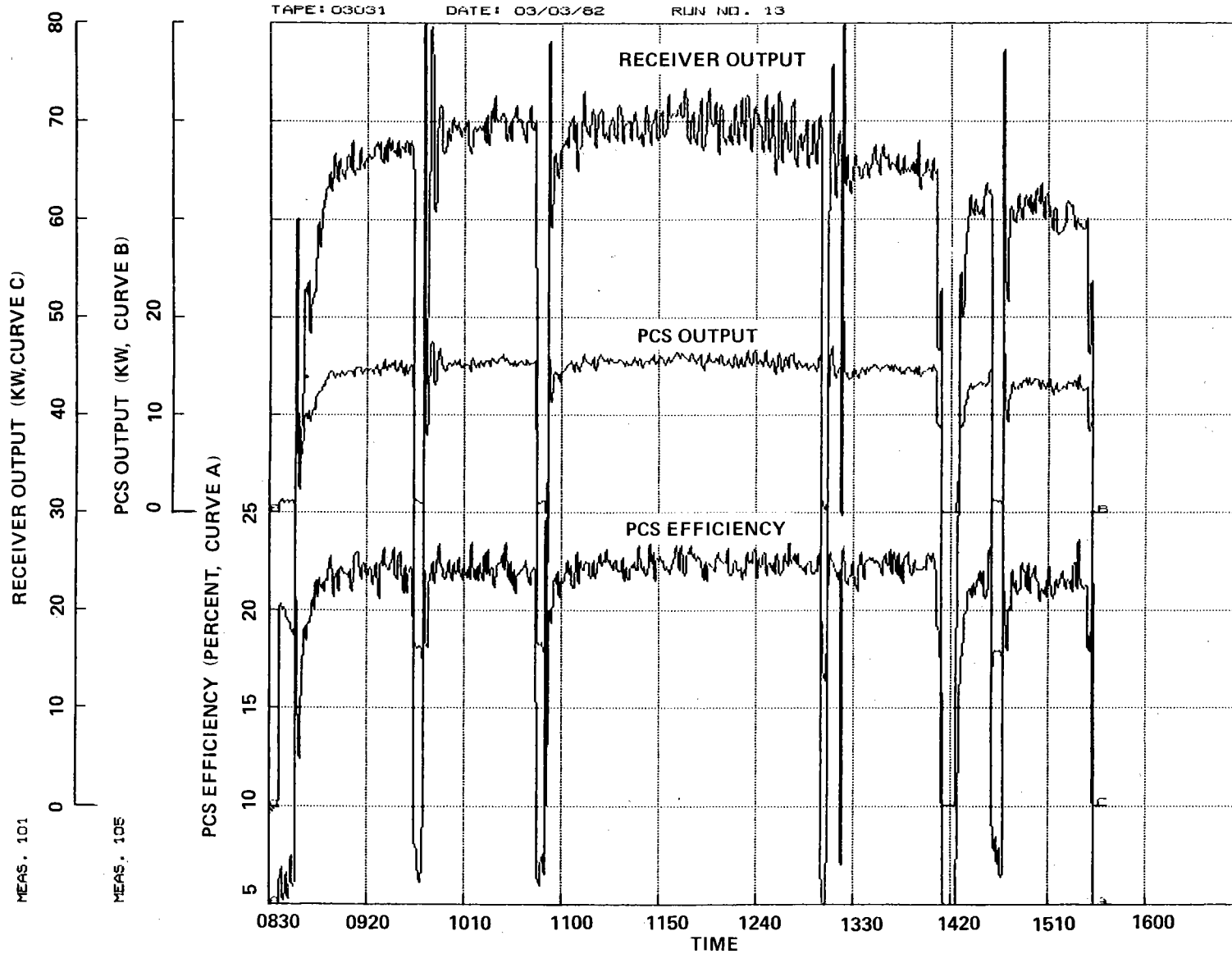
Figure 4-9. Power-Conversion Subsystem Performance History for Run 13 (Test No. 8)
