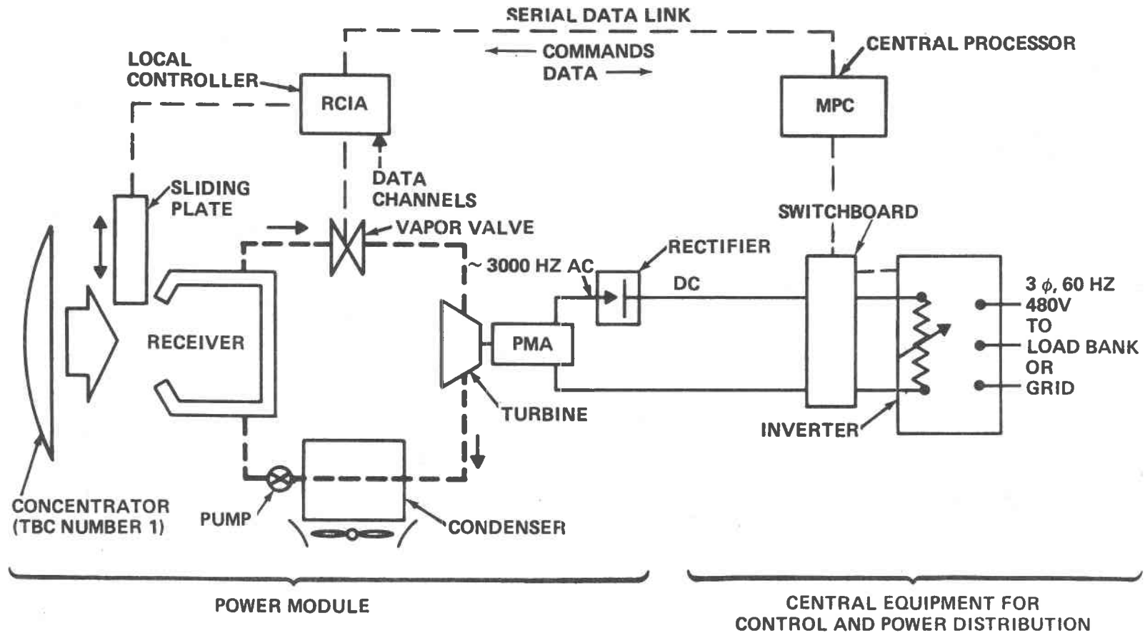
Figure 4-3. Simplified Schematic Diagram of Single-Module Experiment Hardware at Parabolic Dish Test Site
