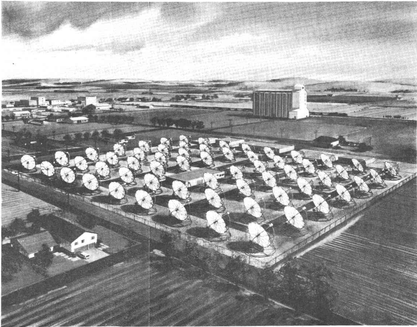
One-Megawatt Experimental Plant Originally Proposed for the Small Community Solar Thermal Power Experiment (SCSE)
