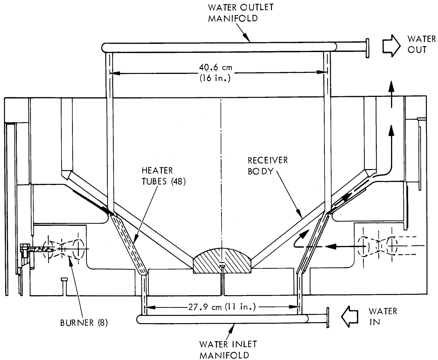
FIGURE 6. DSSR COMBUSTOR TEST RIG
