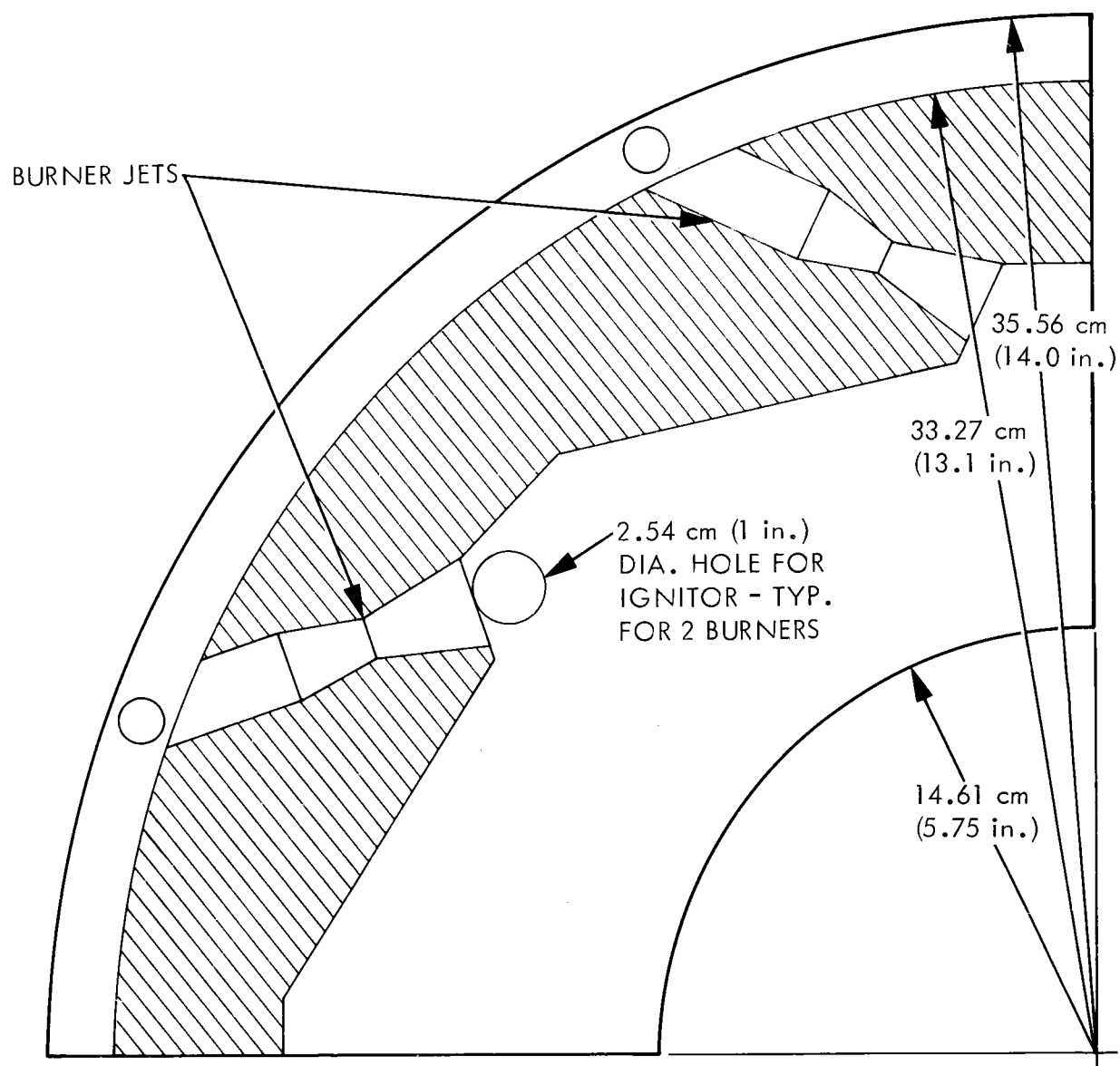
FIGURE 2. COMBUSTOR QUADRANT CROSS-SECTION (PLAN VIEW)
