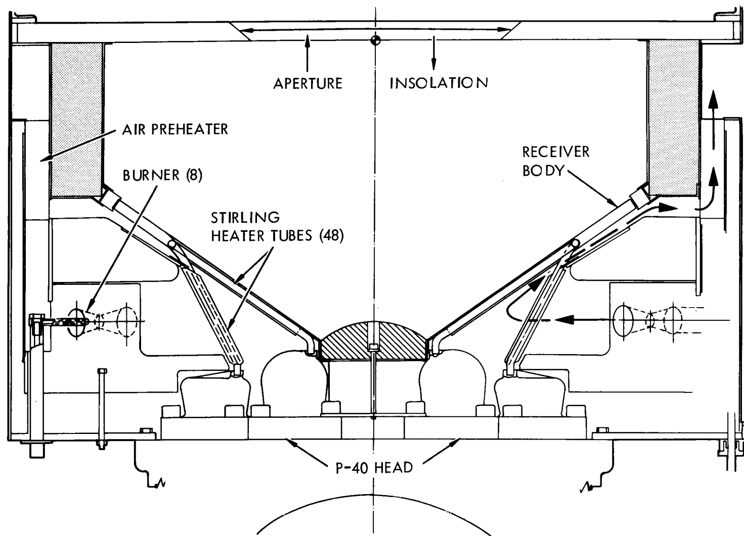
FIGURE 1. DISH STIRLING SOLAR RECEIVER
