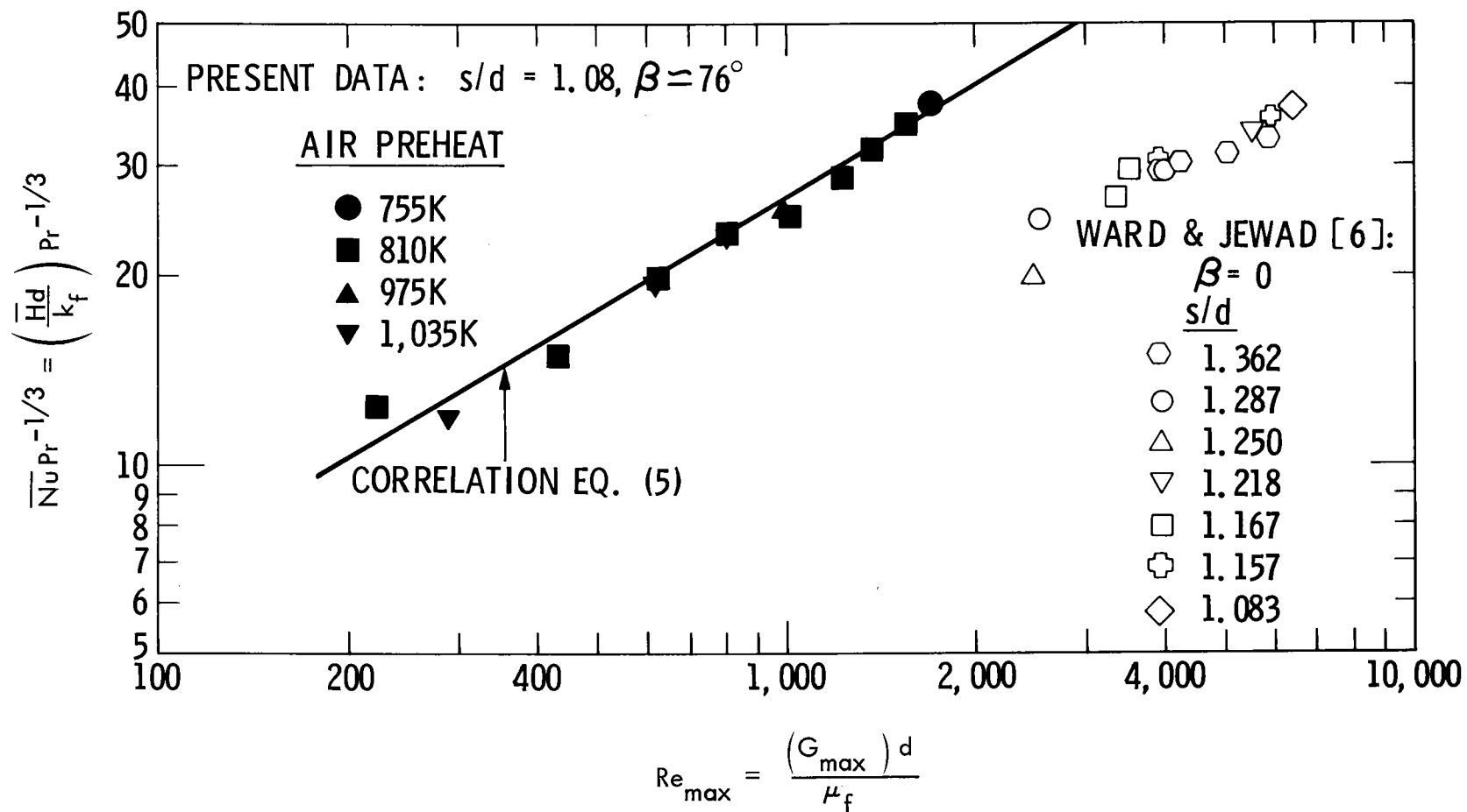
FIGURE 8. AVERAGE GAS SIDE HEAT TRANSFER COEFFICIENTS
