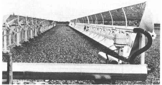
Single-Axis Tracking Parabolic Troughs at the Small Solar Power System Project
