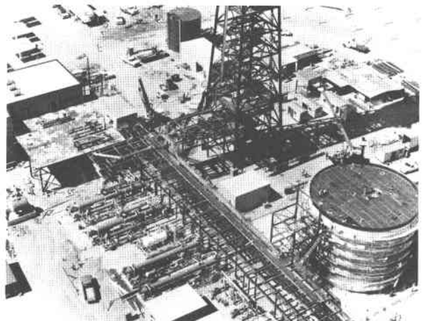
Aerial View of Storage, Piping and Control Room at 10-MWe Solar Central Receiver Pilot Plant
