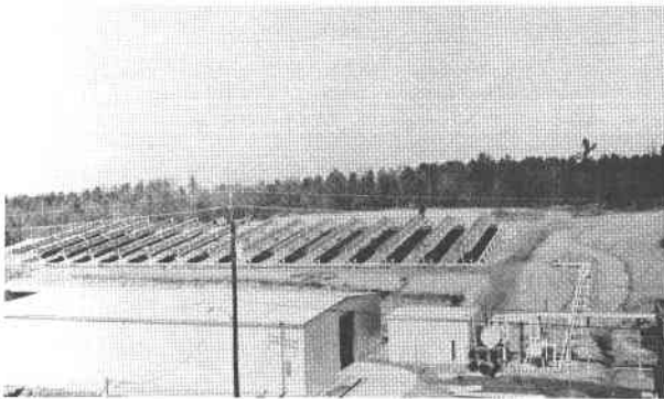
Parabolic Troughs Installed at Dow Chemical Plant in Dalton, Georgia
