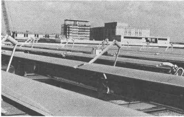
Roof-Mounted Parabolic Troughs at Lone Star Brewery, San Antonio, Texas
