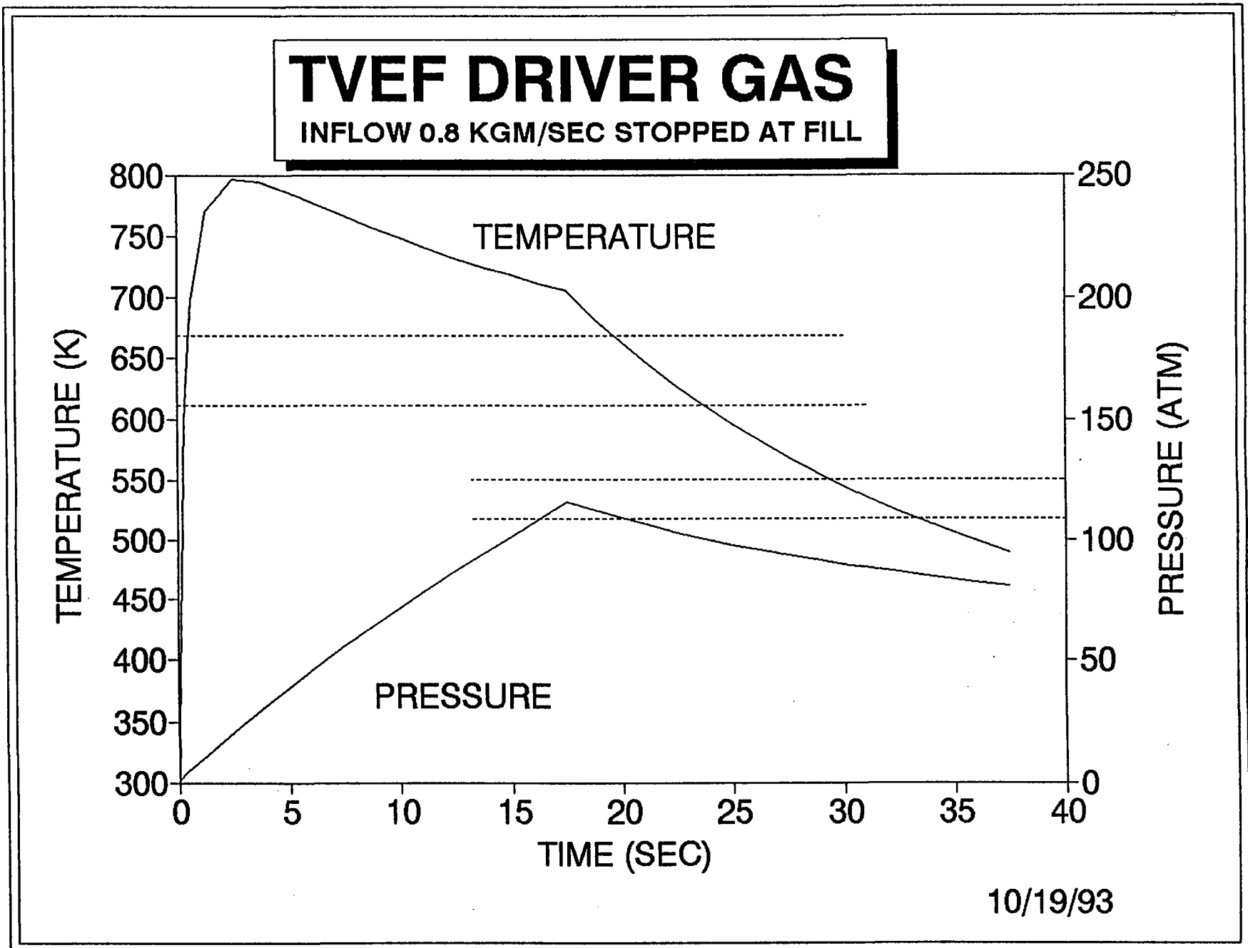
Figure 12. Effect of Terminating Driver Gas Filling
