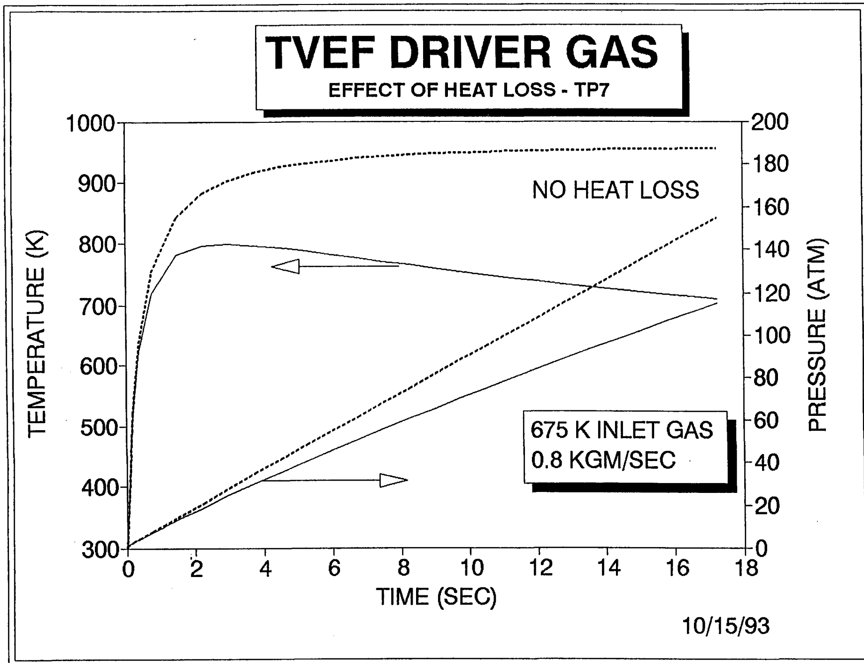
Figure 11. Effect of Heat Transfer to the Driver Wall
