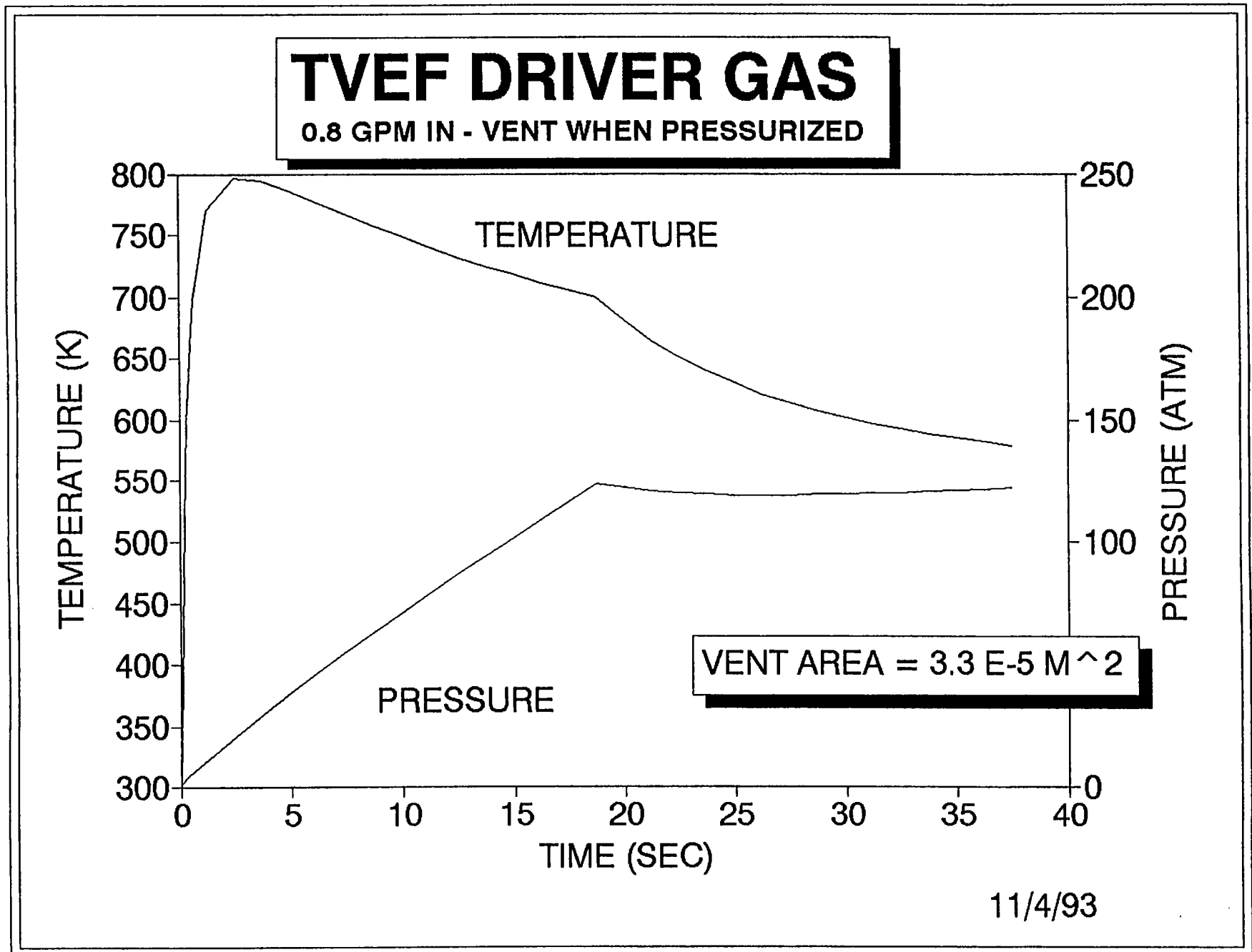
Figure 13. Extending Test Time by Driver Gas Venting
