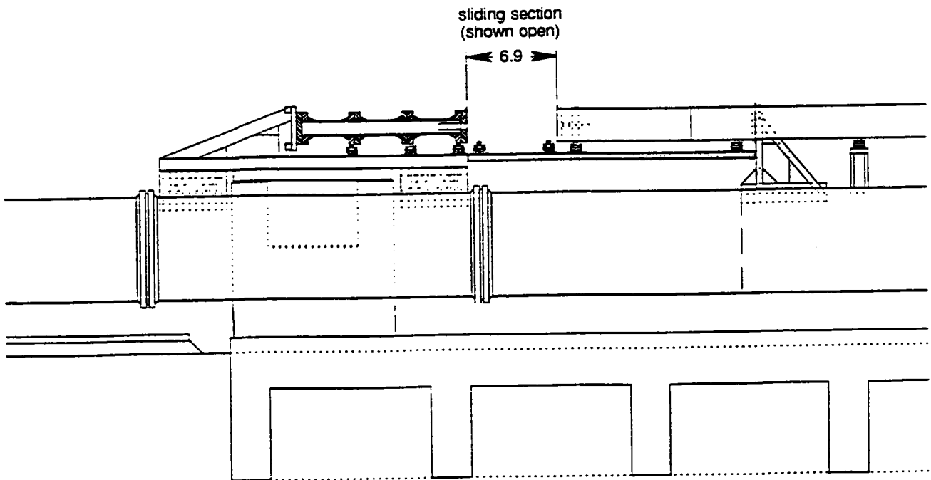
Figure 5. Mobile Work Platform and Sliding Expansion Tube Detail
