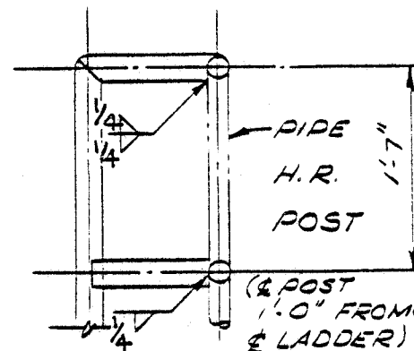
SIDE ELEVATION WITH HANDRAIL
