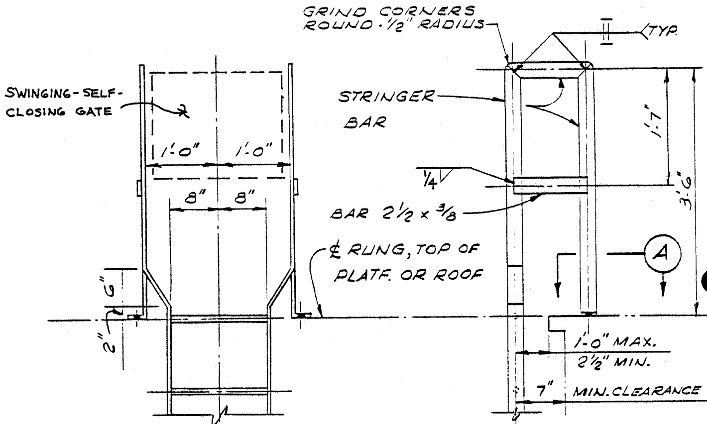
SIDE ELEVATION WITHOUT HANDRAIL
