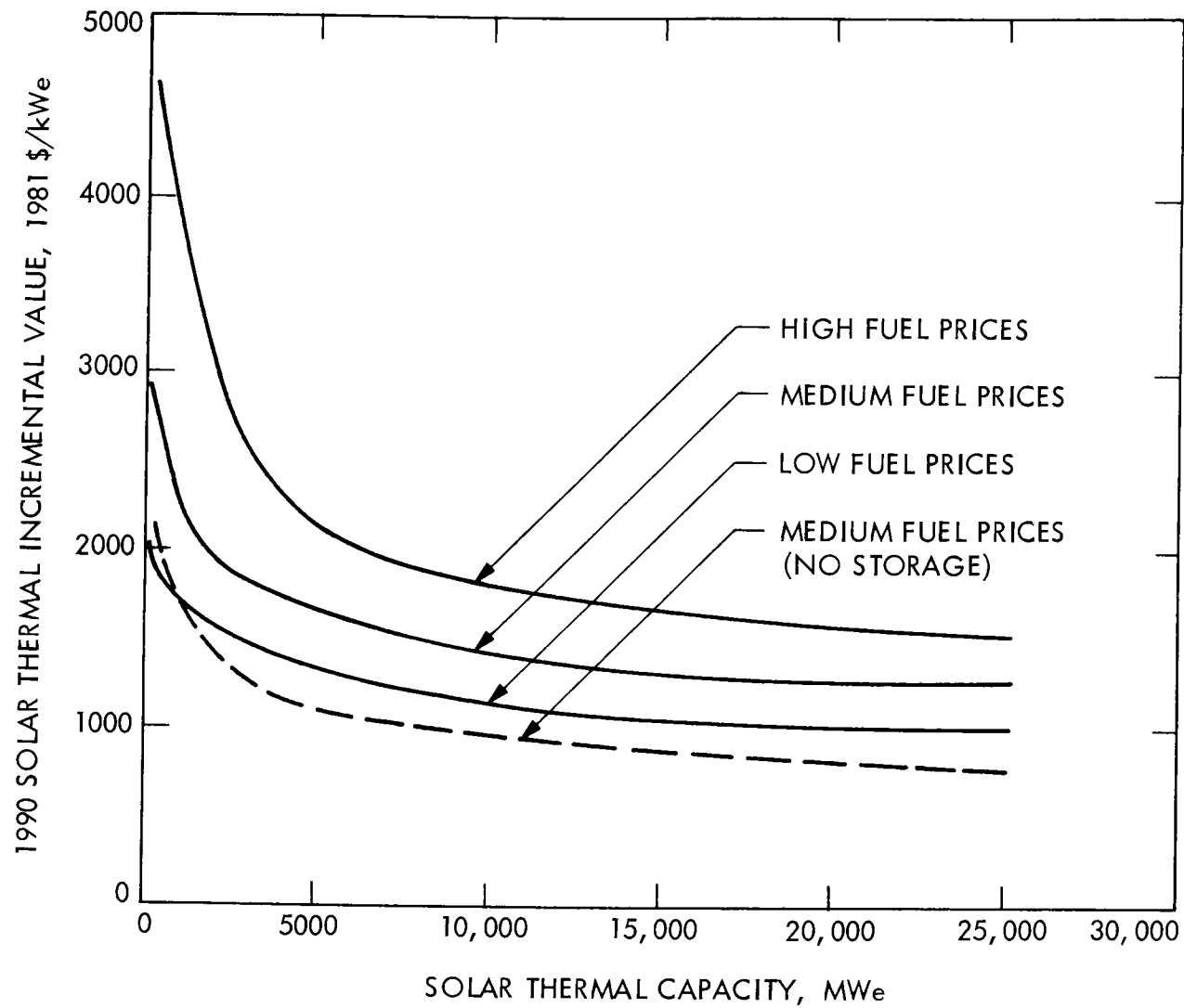
Figure 7-6. 1990 Incremental Value of STT with Storage (Investor-Owned Utilities; Southwest and South Central Regions)
