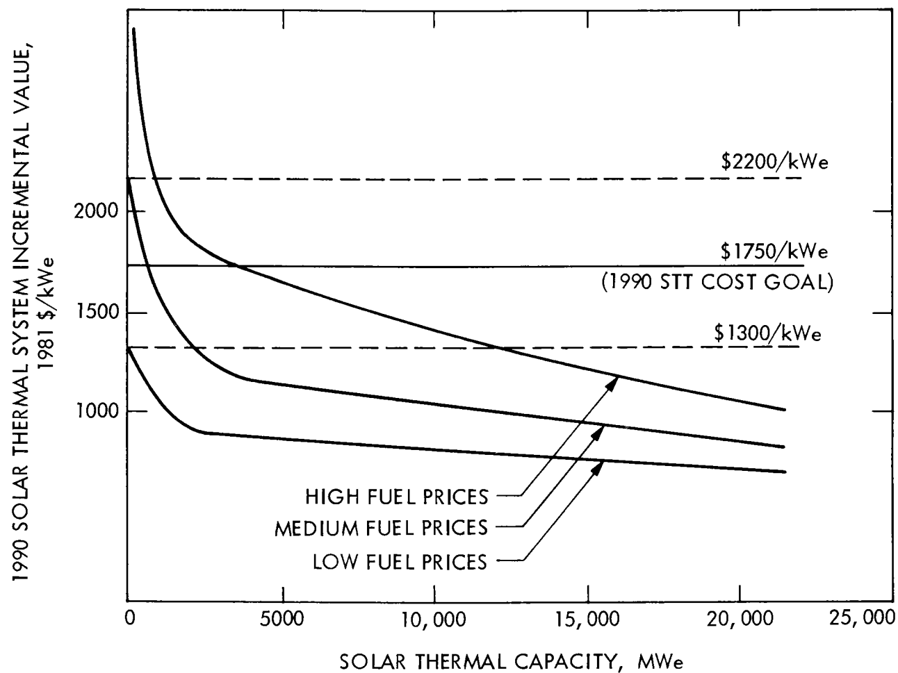
Figure 6-1. 1990 Market Potential for Cost-Competitive Solar Thermal Electric Systems (Investor-Owned Utilities; Southwest and South Central Regions; No Storage; After Tax Incremental Values)
