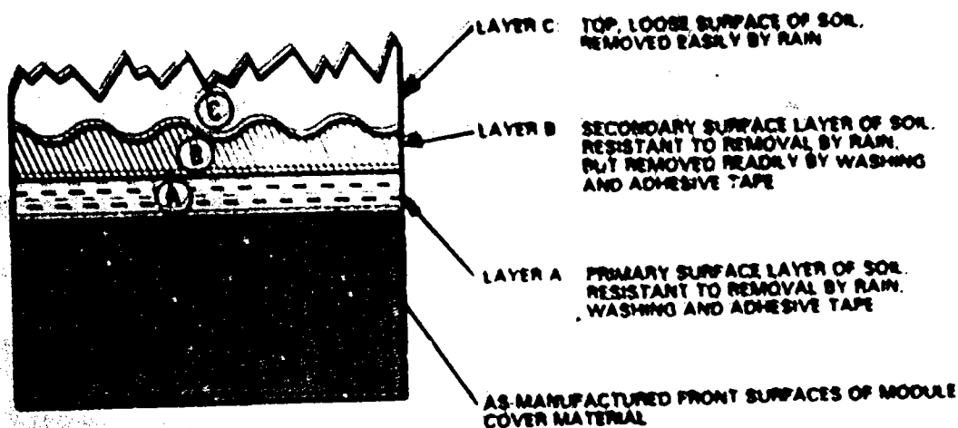
Figure 1: The Three Soiling Layers
