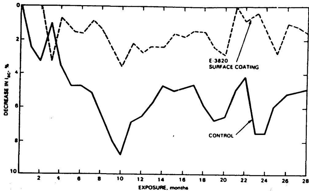
Figure 7. Outdoor Soiling Behavior of Tedlar 100BG3OUT Plastic Film, With and Without a Fluorocarbon Antisoiling Coating
