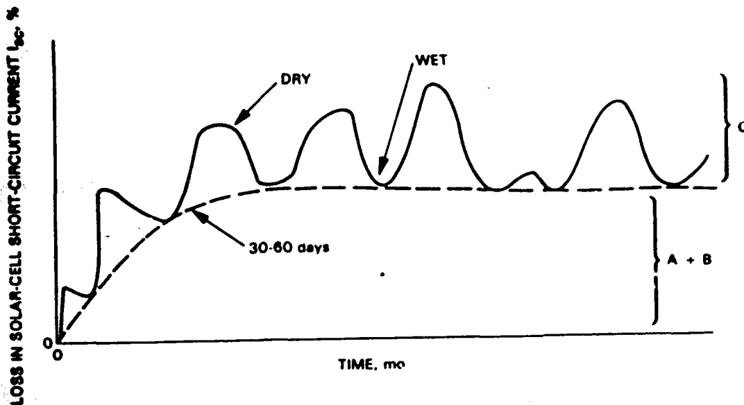
Figure 2. Behavior of Natural Outdoor Soiling
