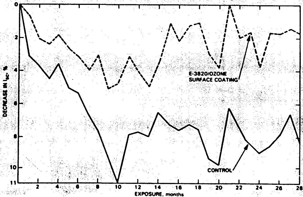
Figure 8. Outdoor Soiling Behavior of Acrylar X-22417 Plastic Film, With and Without a Fluorocarbon Antisoiling Coating
