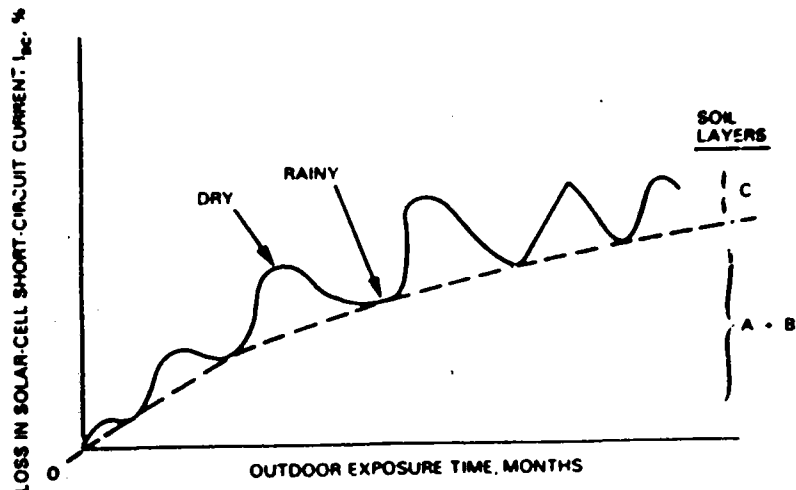
Figure 3. General Pattern Observed in JPL Outdoor Soiling Data for GE RTV-615 Soft Silicone at Point Vicente, Goldstone and Table Mountain, California
