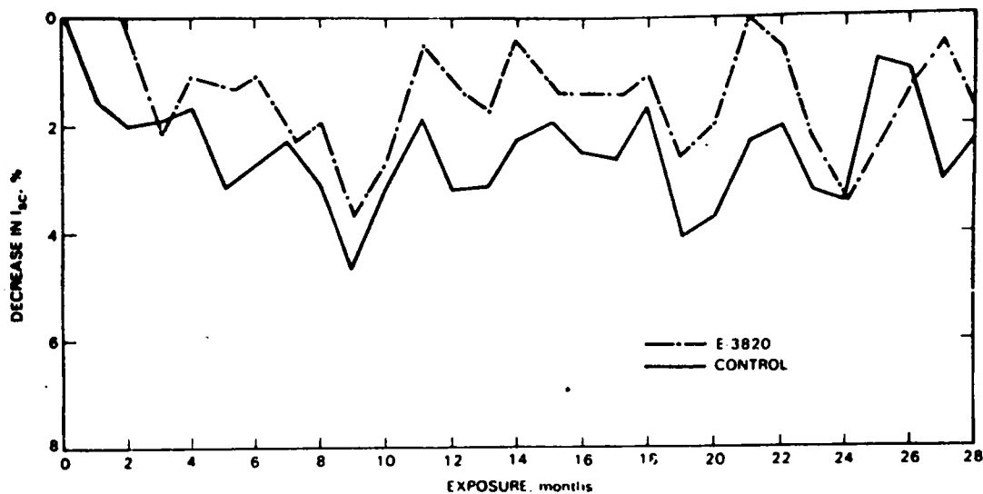
Figure 9. Outdoor Soiling Behavior of Glass With and Without a Fluorocarbon Antisoiling Coating
