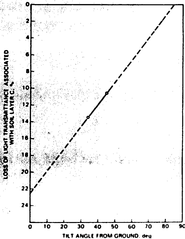
Figure 4. Effect of Tilt Angle on Accumulation of Soil Layer C (Data From Table 1, JPL Sites)
