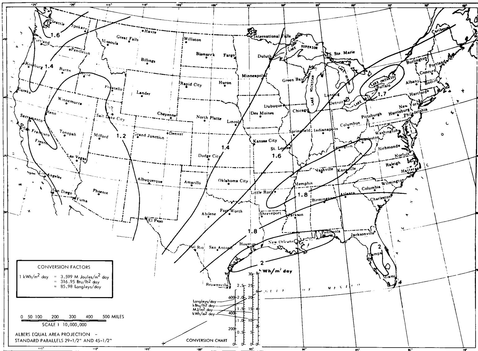
Figure A-5. Annual Average Daily Diffuse Horizontal Insolation in the United States as Presented by Watt Engineering, Ltd
