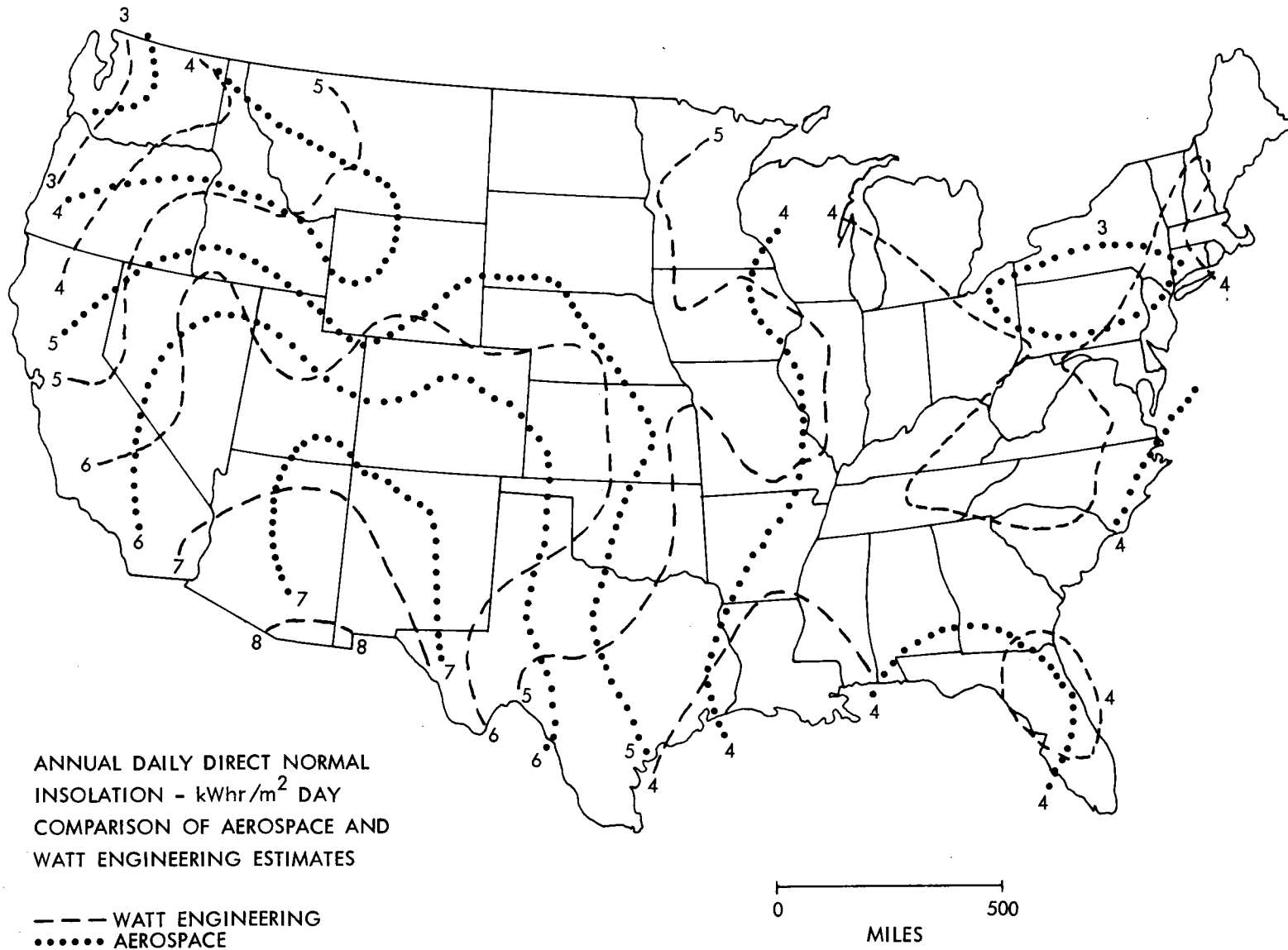
Figure A-7. Annual Average Daily Direct Insolation Contours as Determined by the Aerospace Model and by the Watt Model
