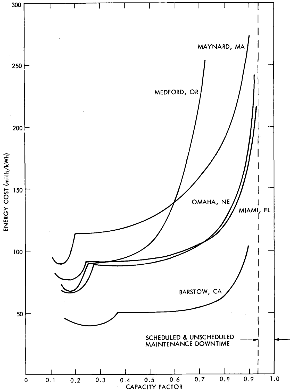
Figure B-5. Minimum Energy Cost Envelopes for the Central Receiver System
