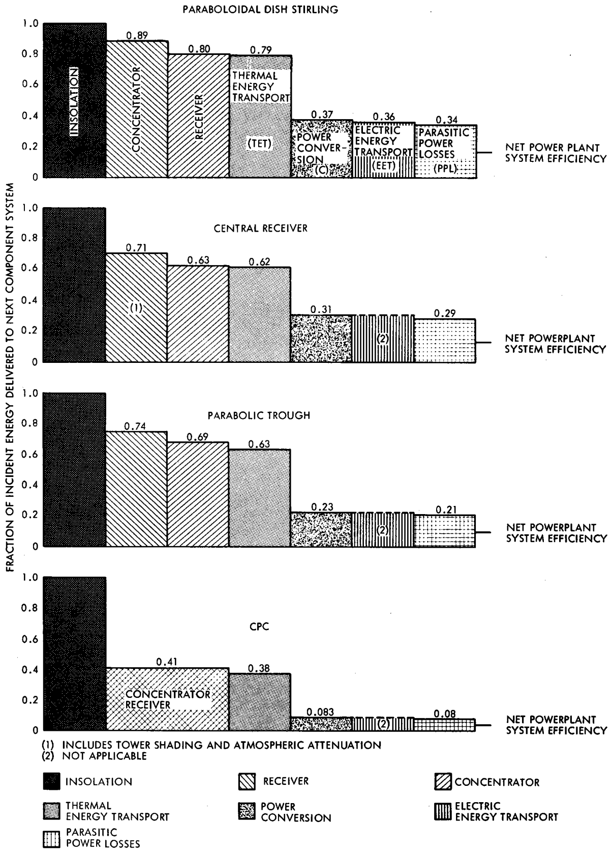
Figure B-1. System Design Efficiency Train
