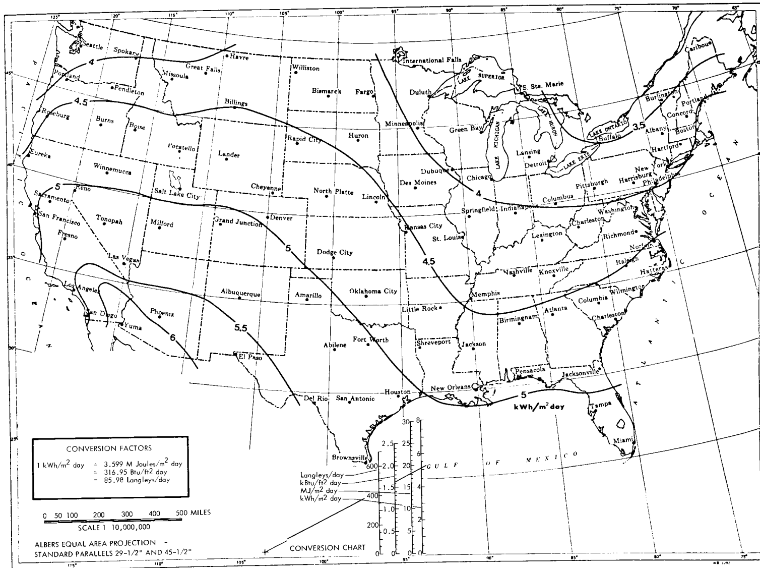
Figure A-6. Annual Average Daily Total Horizontal Insolation in the United States as Presented by Watt Engineering, Ltd
