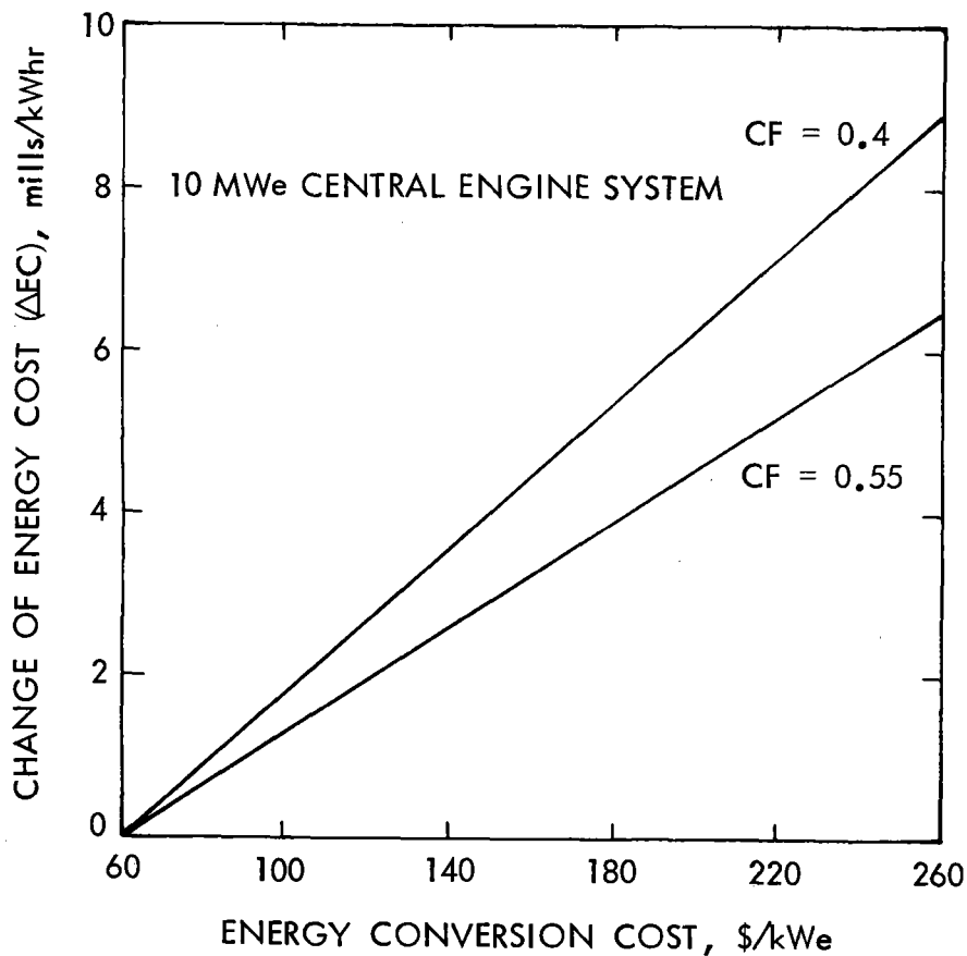
Figure C-3. Sensitivity to Energy Conversion Cost
