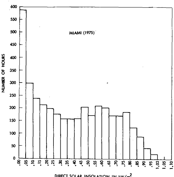
Figure A-19. Histograms of the Annual Hourly Average Direct Insolation for the Same Years and for the Same Sites Presented in Figure A-18.
