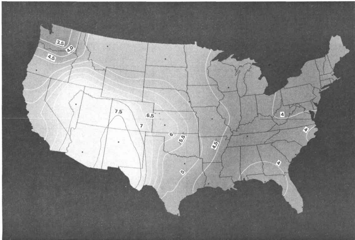
Figure A-15. Data Based on Aerospace Corp. Estimates of Direct Normal Insolation. The Degree of Smoothing of the Surface Increases in Going from Figure A-15 to Figure A-17. Figure A-16 Corresponds Approximately to an Average Nyquist Sampling (See Text).
