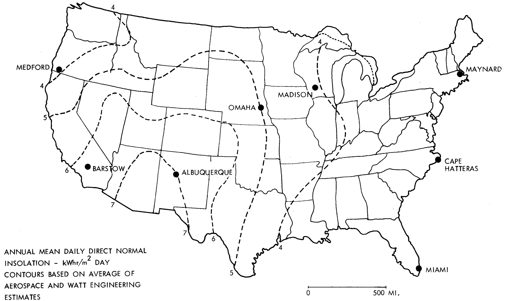
Figure 1. Insolation Patterns and Selected Sites
