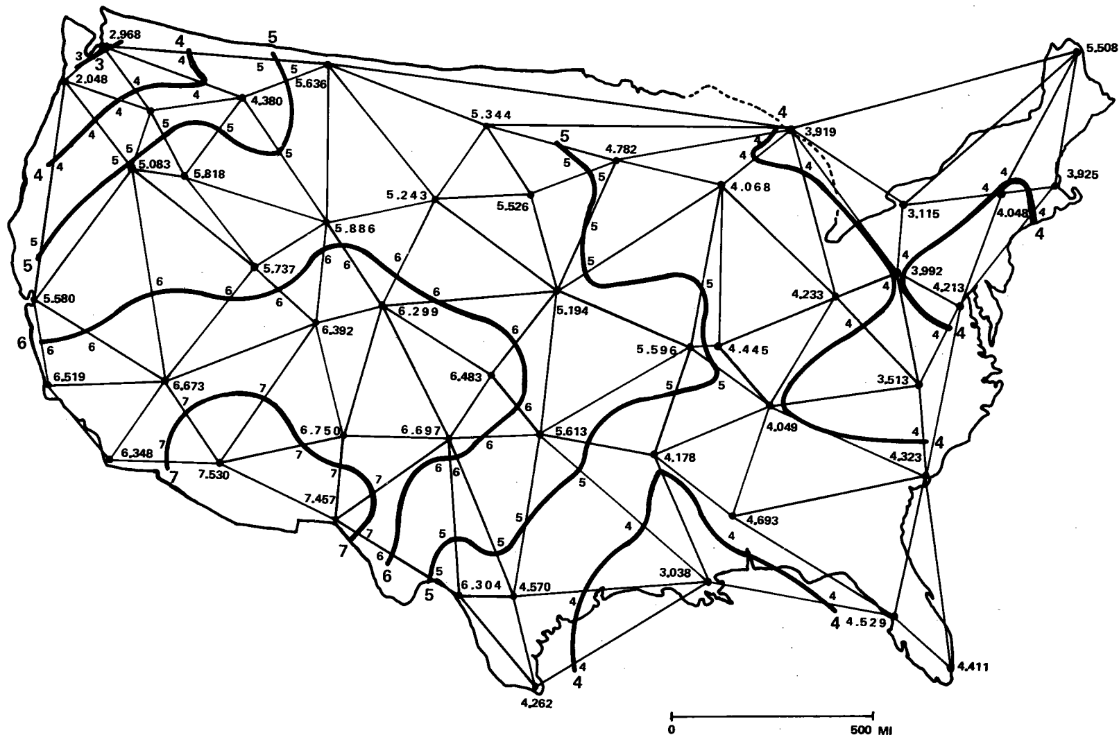
Figure A-8. Annual Mean Daily Direct Normal Insolation (Watt data, linearly interpolated)
