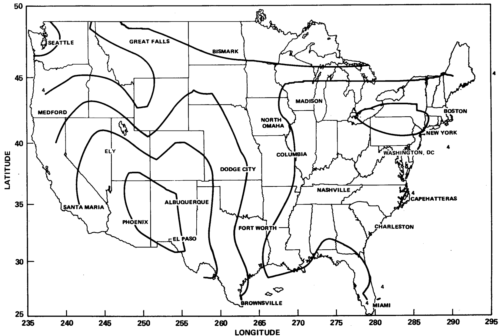
Figure A-11. Annual Mean Daily Direct Normal Insolation (Aerospace data, cubic spline fitted)
