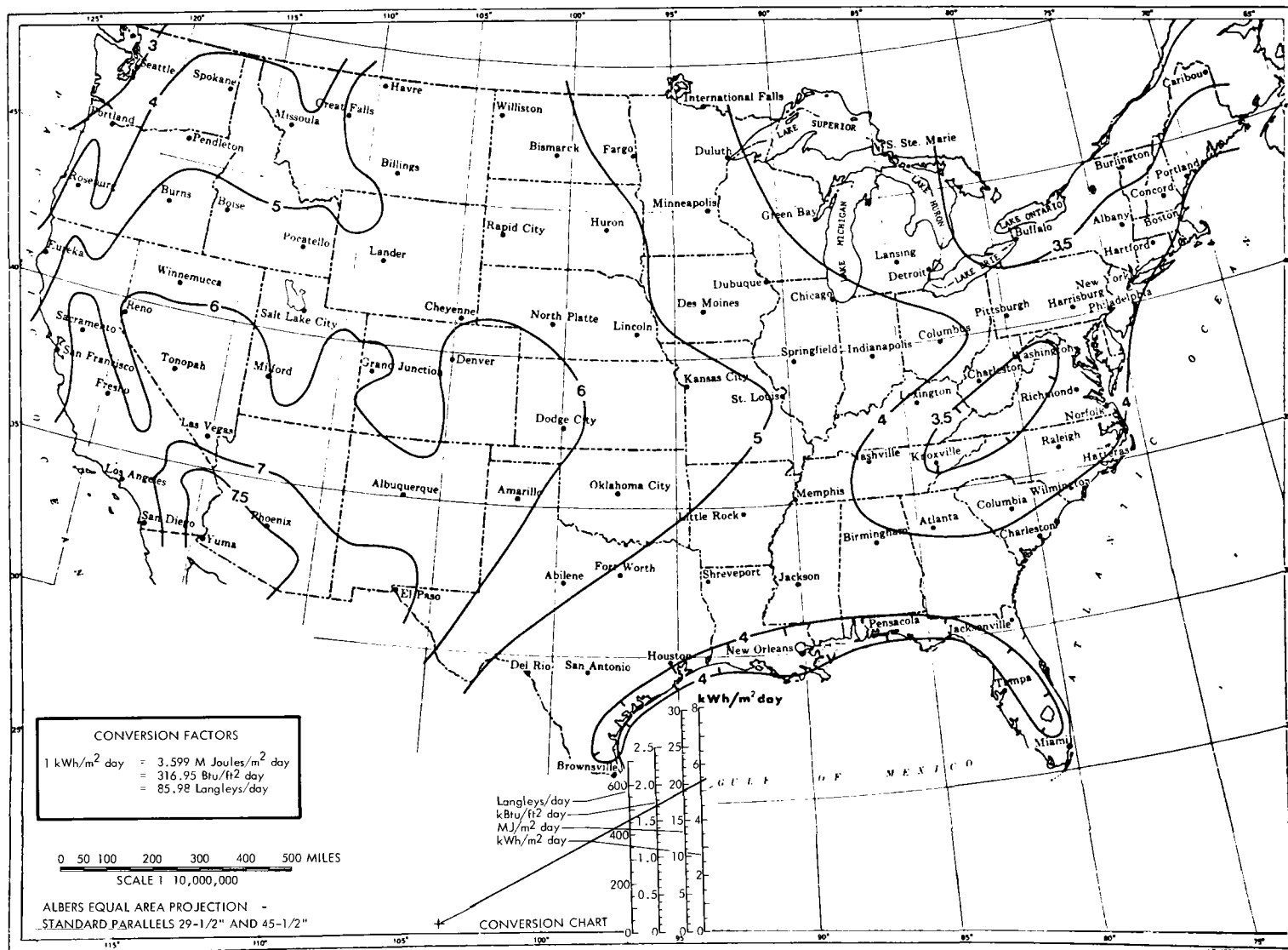
Figure A-4. Annual Average Daily Direct Normal Insolation in the United States as Presented by Watt Engineering, Ltd.
