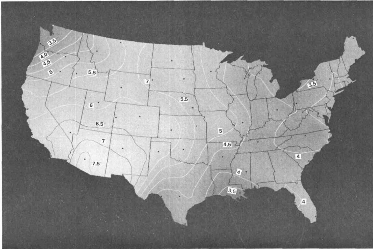
Figure A-14. Data Based on Watt Engineering, Ltd. Estimate of Direct Normal Insolation. The Degree of Smoothing of the Surface Increases in Going from Figure A-12 to Figure A-14, Figure A-13 Corresponding Approximately to an Average Nyquist Sampling (See Text).
