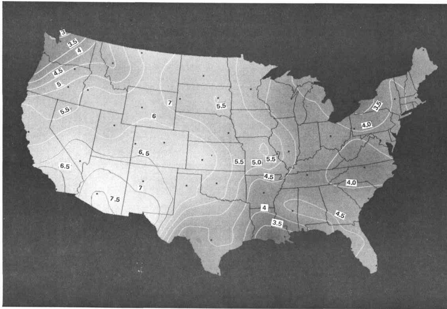
Figure A-13. Data Based on Watt Engineering, Ltd. Estimate of Direct Normal Insolation. The Degree of Smoothing of the Surface Increases in Going from Figure A-12 to Figure A-14. Figure A-13 Corresponding Approximately to an Average Nyquist Sampling (See Text).
