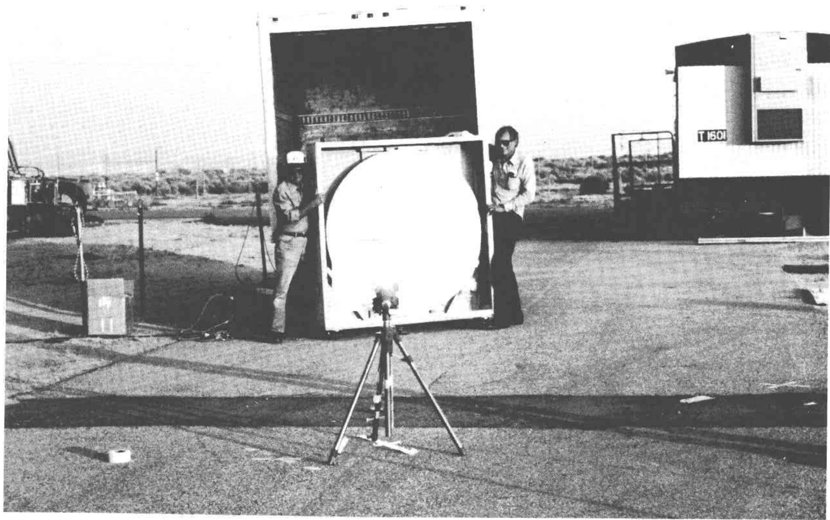
Figure 5. Test Configuration for Sun Tests
