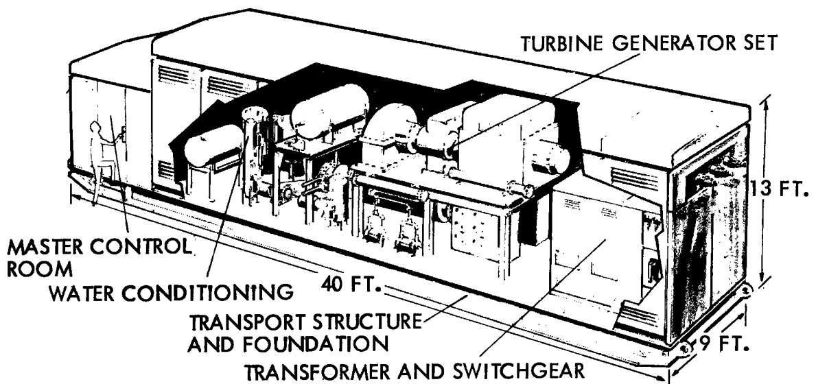
Figure V-8. GE Power Conversion Module Concept
