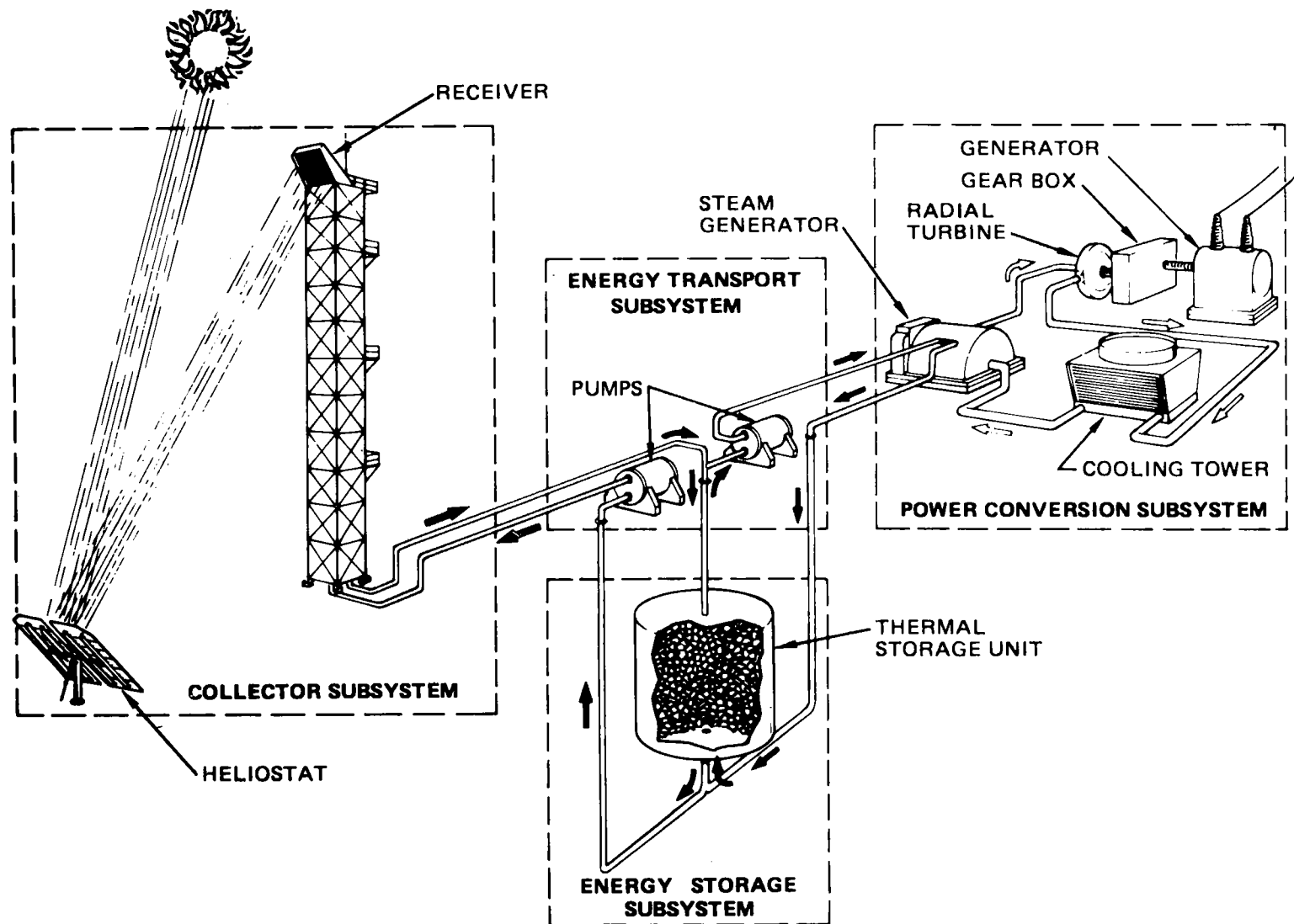
Figure V-3. System Schematic Diagram for McDonnell-Douglas Concept
