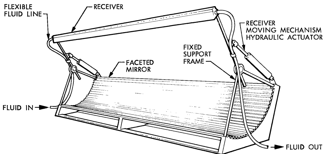
Figure III-8. Line-Focus Distributed Receiver Concept Using Fixed Mirrors and Movable Receivers
