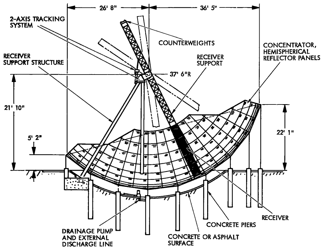
Figure III-7. Fixed Mirror Distributed Focus Concept
