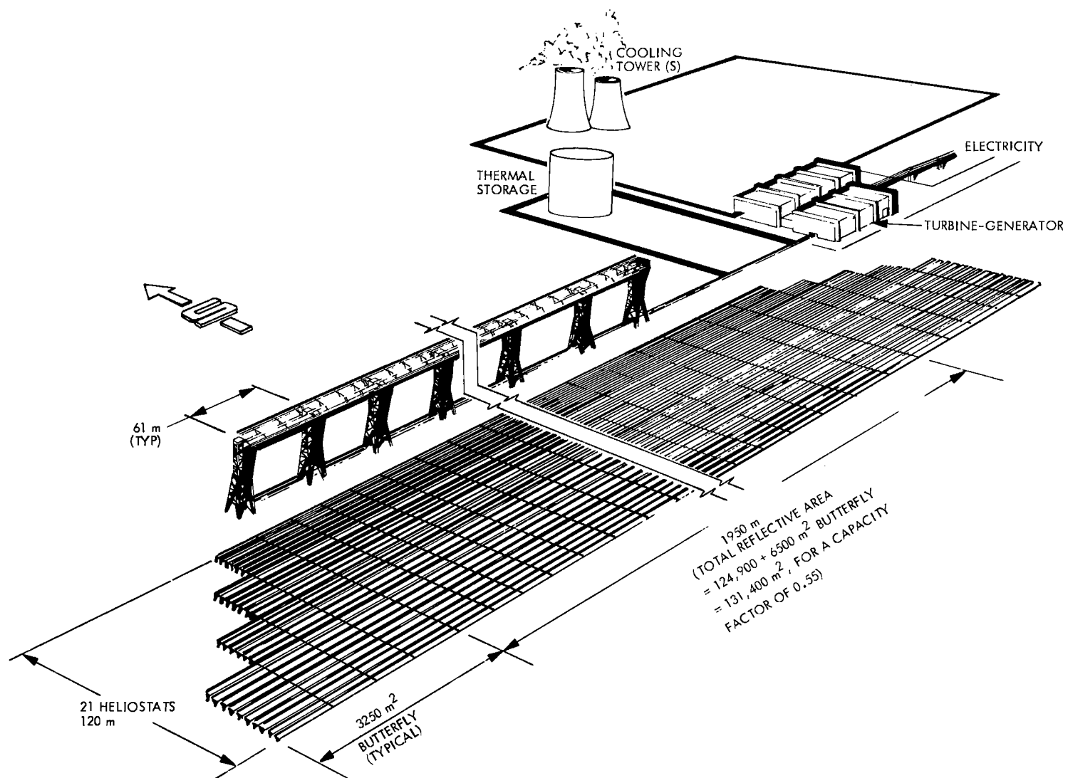
Figure III-6. Line-Focus Central Receiver Concept
