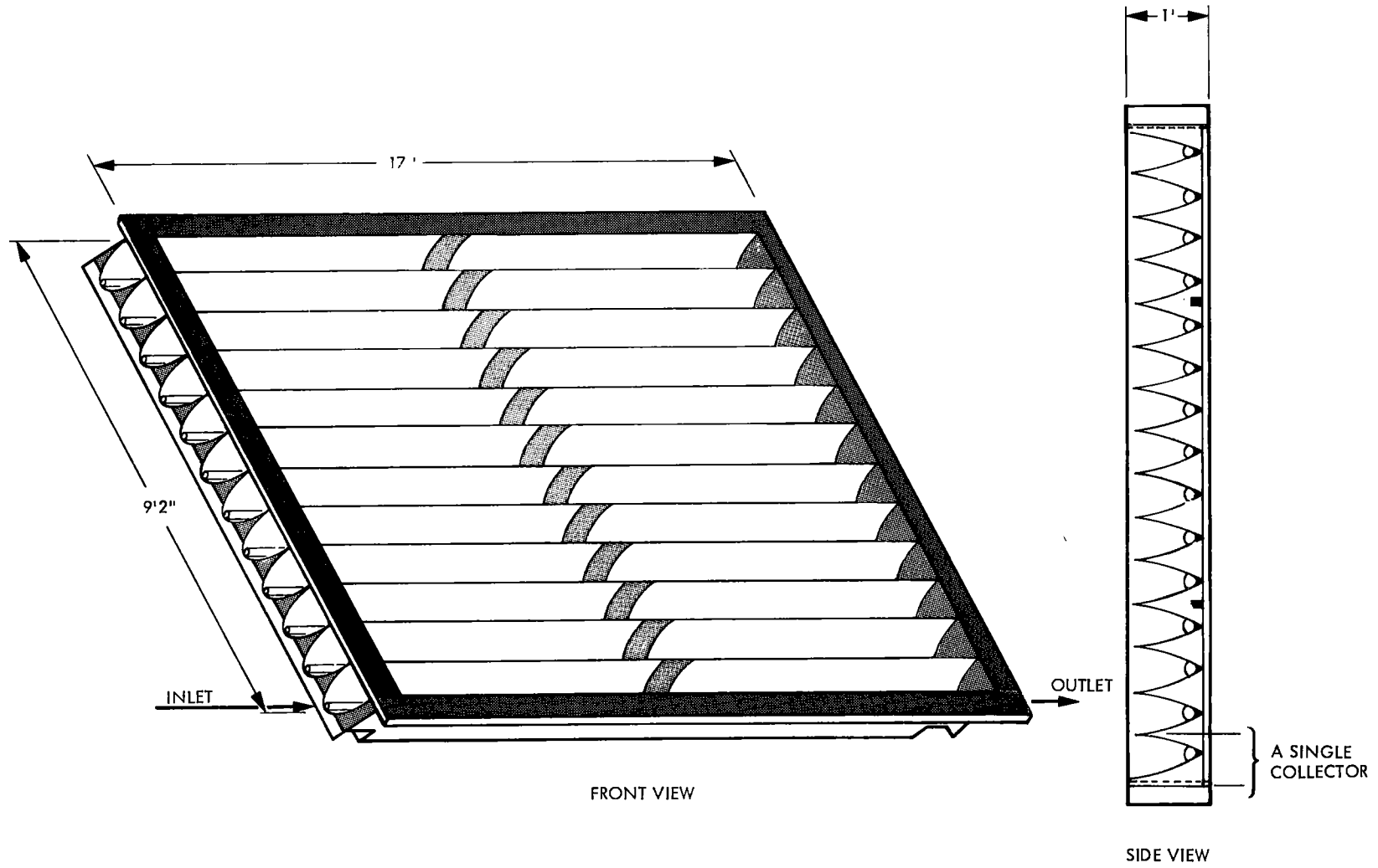
Figure III-9. Low-Concentration Non-Tracking Concept (LCNT)/ Compound Parabolic Concentrator (CPC)
