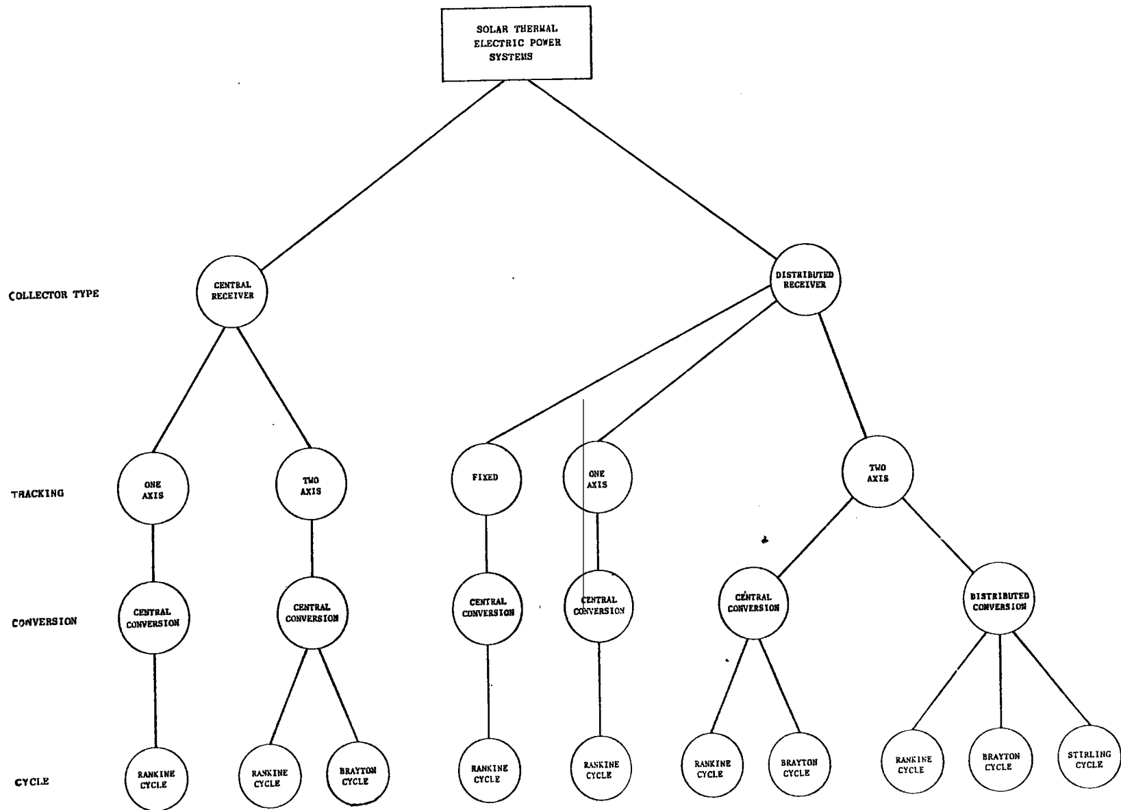
Figure III-10. Breakdown of Solar Thermal Energy Conversion Cycles
