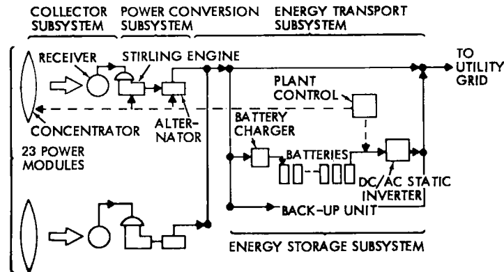
Figure V-10. System Schematic of the Ford Design
