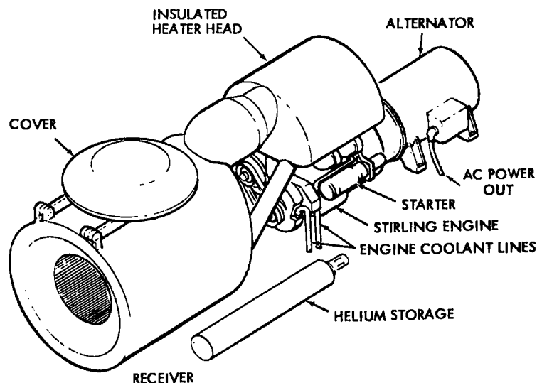
Figure V-11. Receiver Power Conversion Unit for the Ford Design
