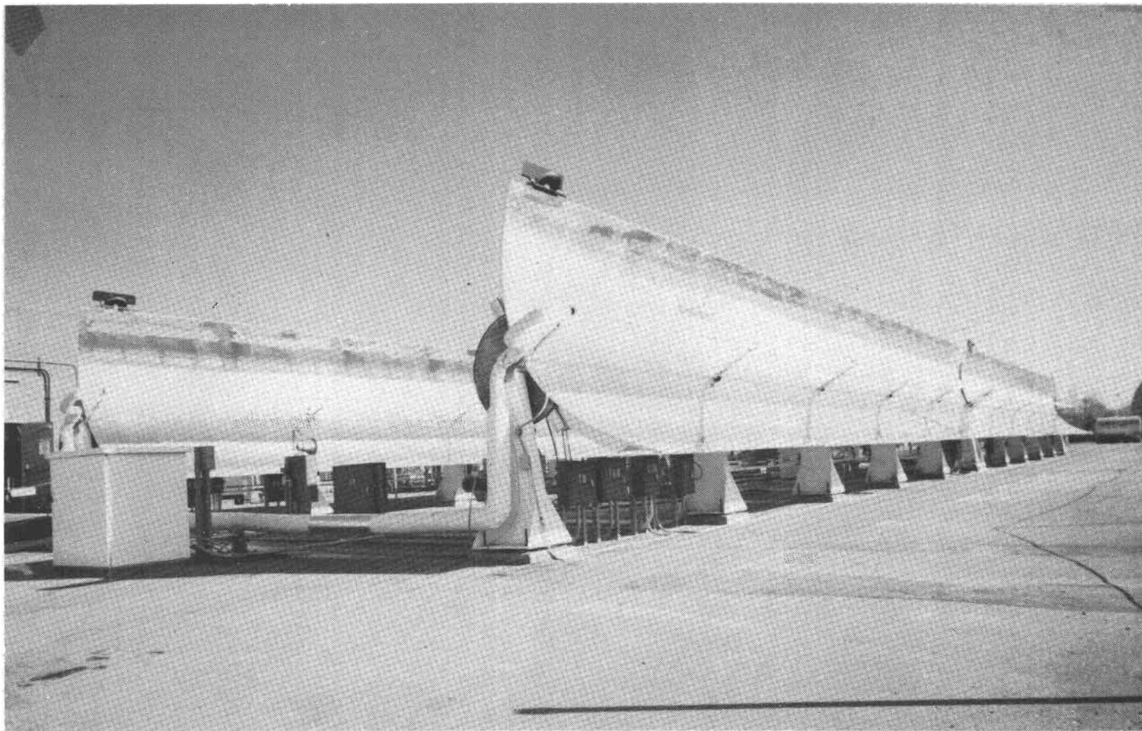
Figure III-4. Line-Focus Distributed Receiver Concept Using Parabolic Troughs
