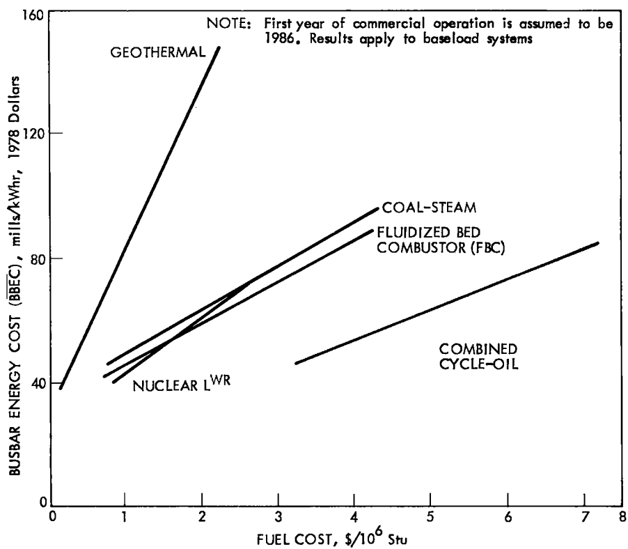
Figure II-2. Sensitivity of Busbar Energy Cost to Fuel Cost
