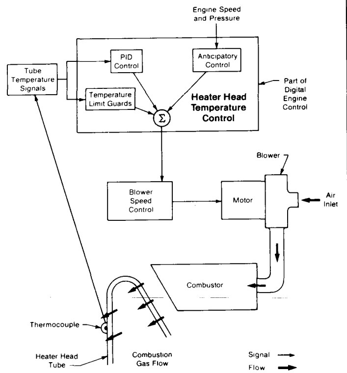
HEATER HEAD TEMPERATURE CONTROL
