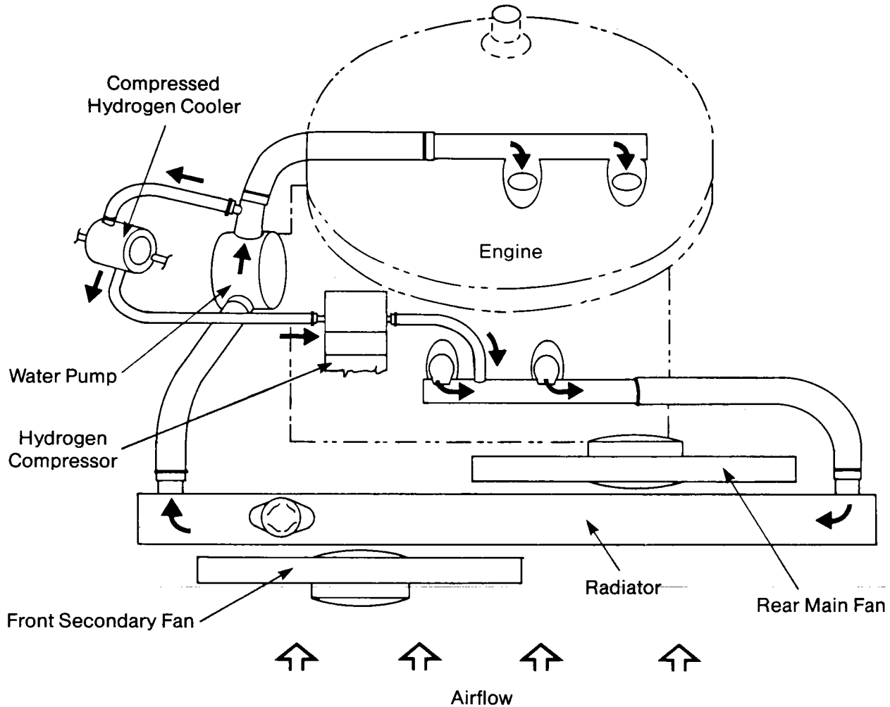
COOLING SYSTEM
