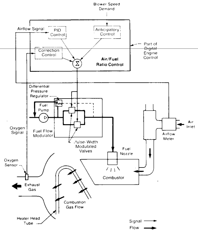
AIR/FUEL RATIO CONTROL
