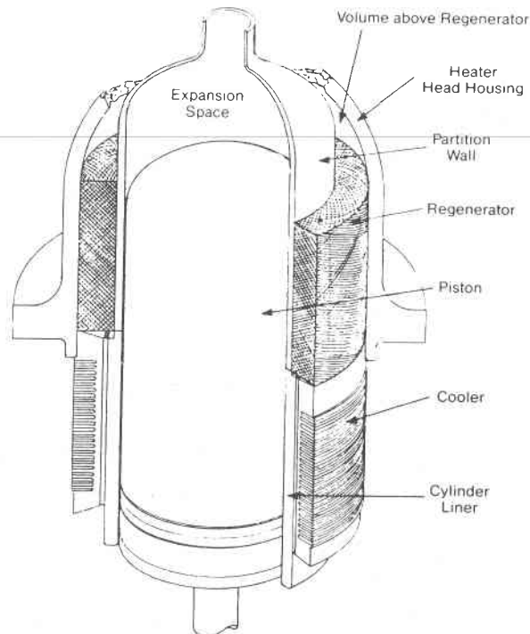
TYPICAL ANNULAR HOT ENGINE SYSTEM
