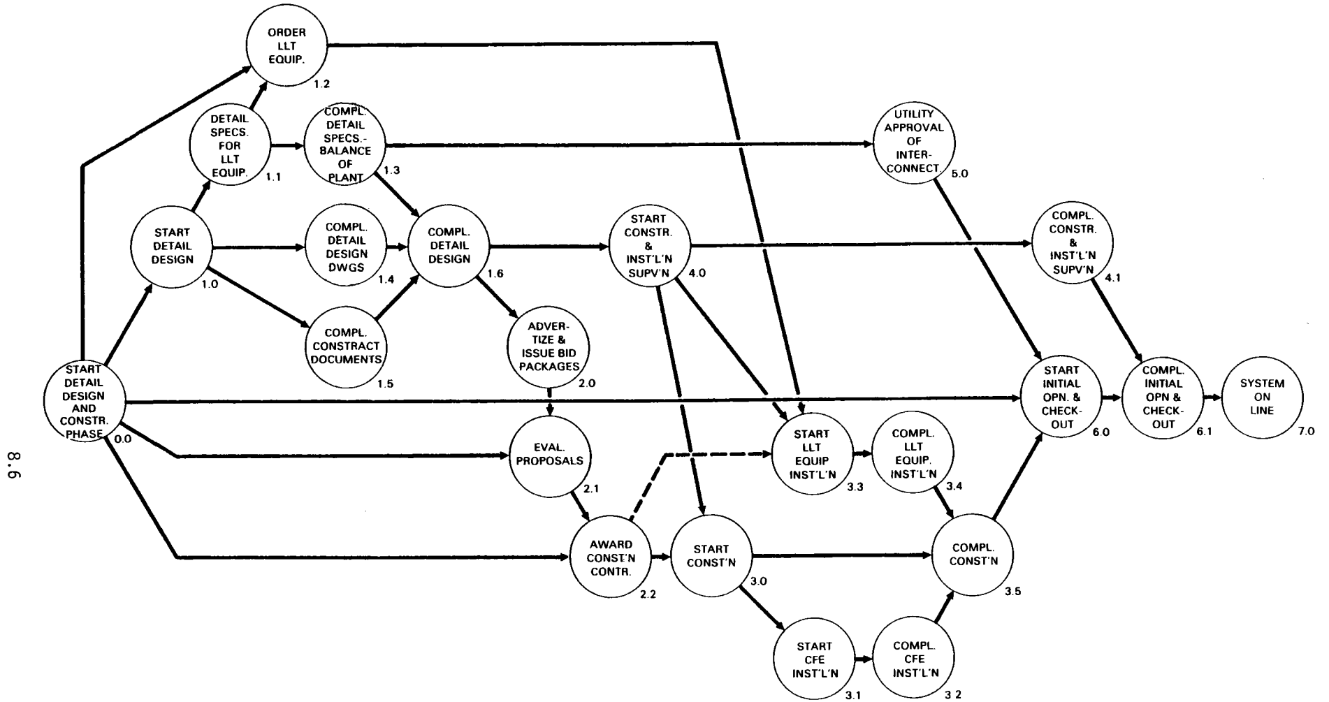
FIGURE 8.3. Detailed-Design-and-Construction Phase
