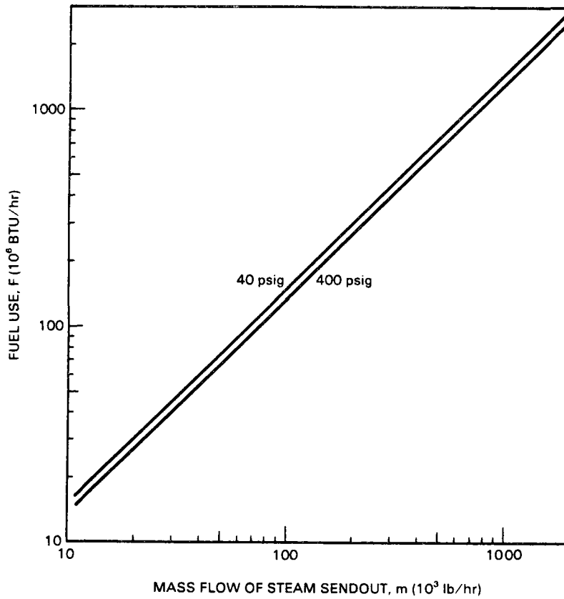
FIGURE 3.6. Steam Turbine Fuel Use
