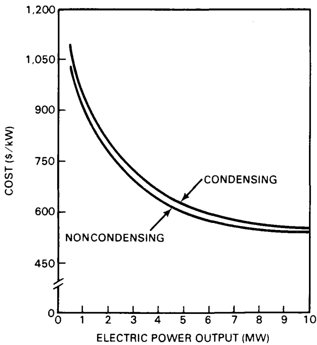
FIGURE F.5. Estimated Installed Costs for Condensing and Noncondensing Steam Rankine Bottoming Systems
