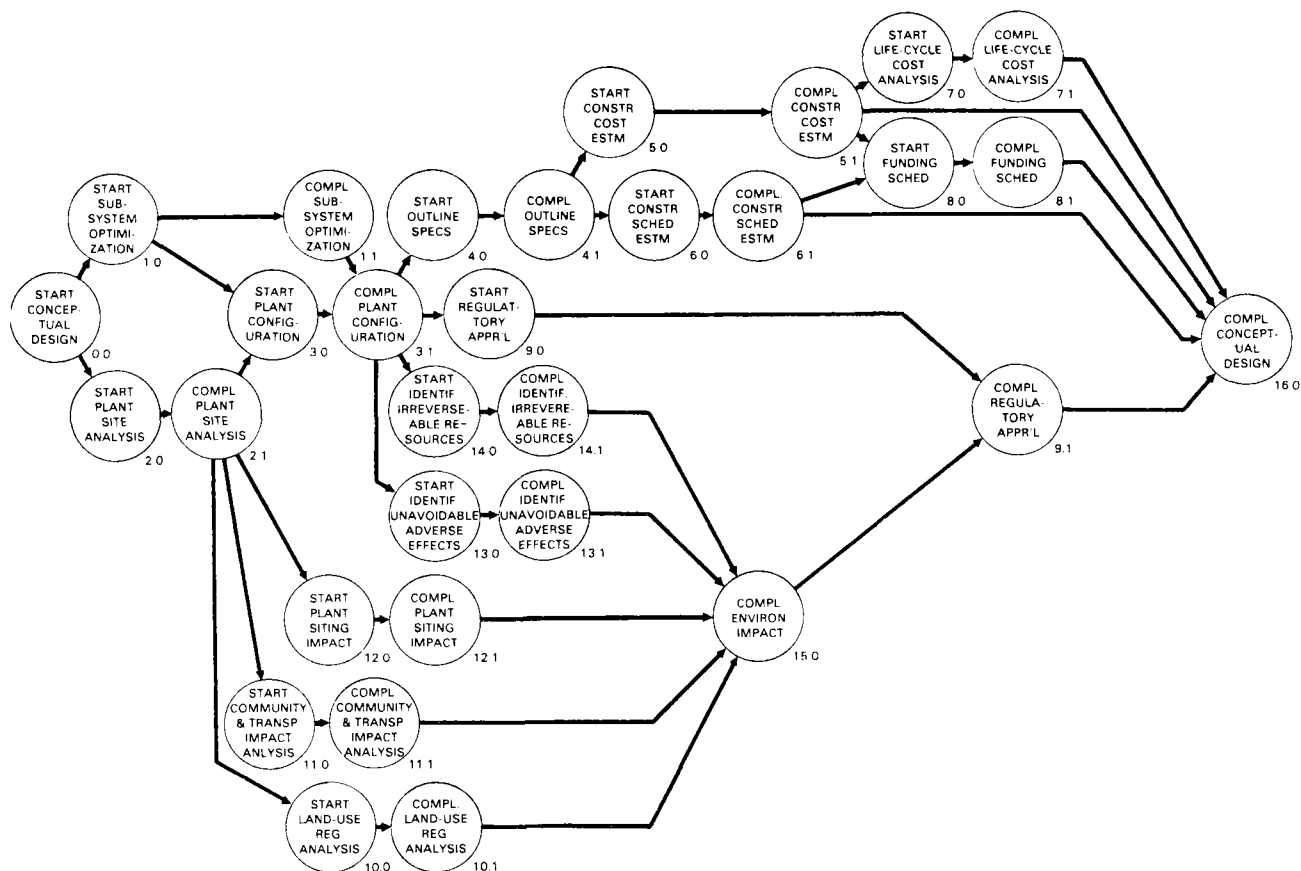
FIGURE 8.2. Conceptual-Design Phase
