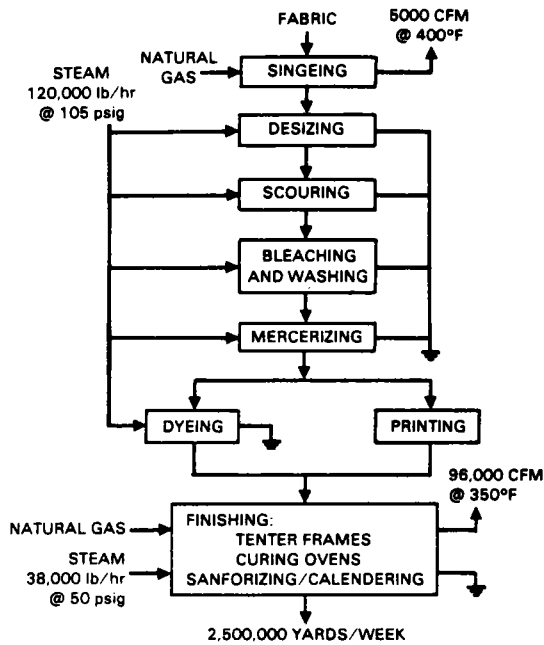
FIGURE 2.2. Finishing Plant Flow Diagram
