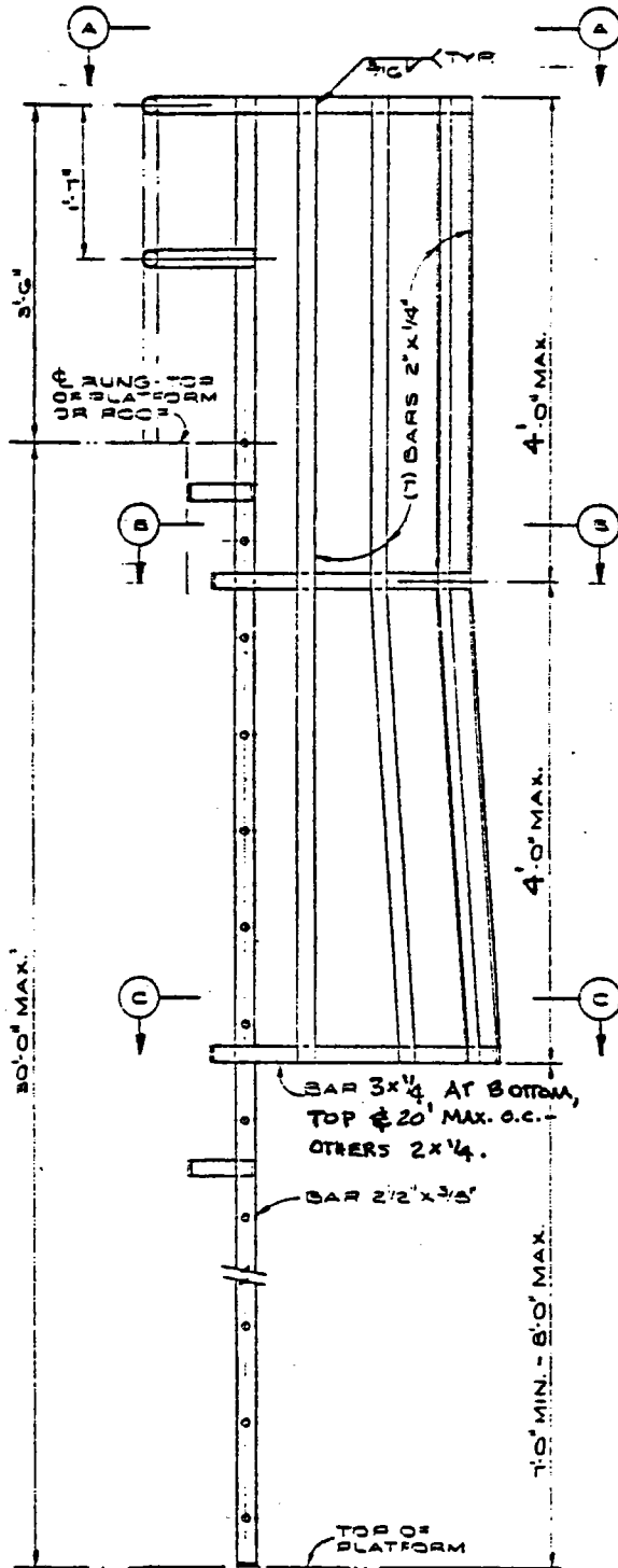
SIDE ELEVATION
