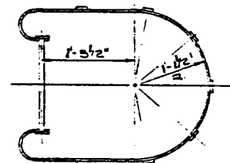
SECTION "C" BOTTOM
