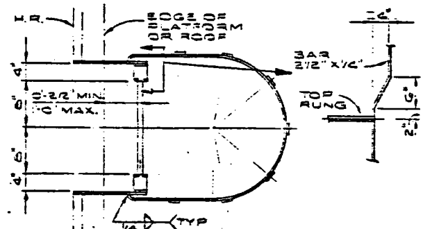
VIEW "A" THRU STEP
