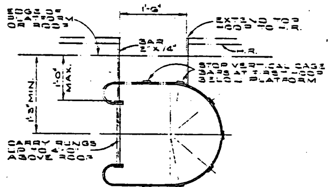
VIEW "A" SIDE STEP
