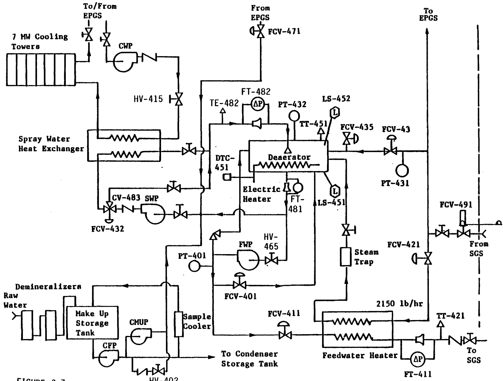
FIGURE 3.7 Heat Rejection and Feedwater Subsystem (HRFS)
