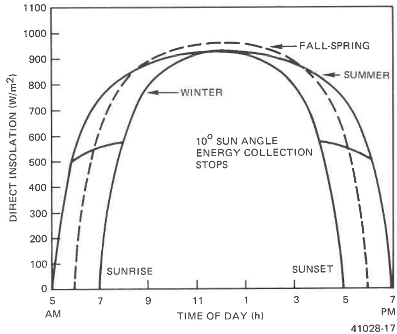
Figure 1-5. Clear Day Solar Insolation
