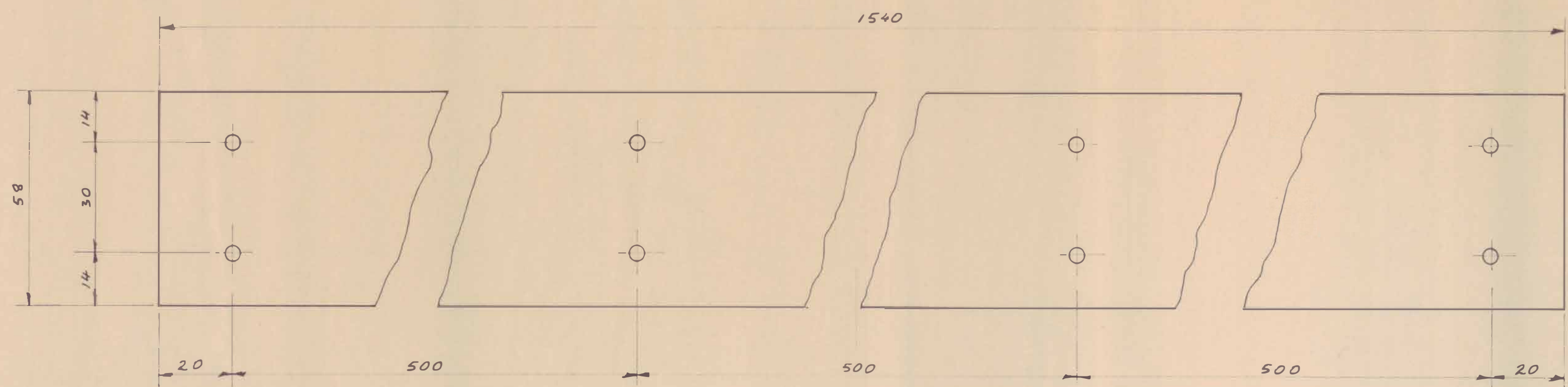
Heat Sink # 18 SWG Cu. 2 off
